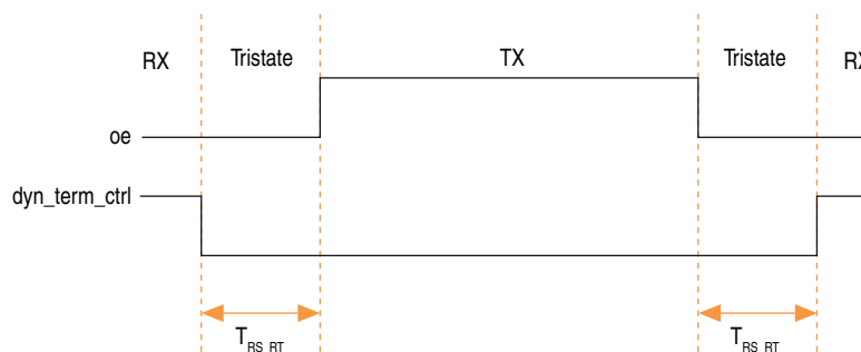
Figure 6. Timing Diagram for oe and dyn_term_ctrl Signals
