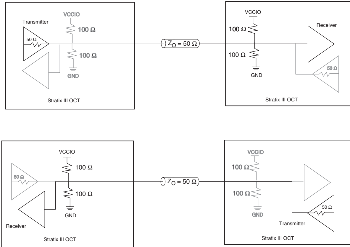
Figure 7–12. Dynamic Parallel OCT in Stratix III Devices
