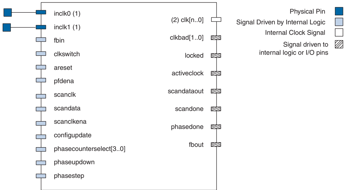
Figure 6–20. Stratix III PLL Ports
