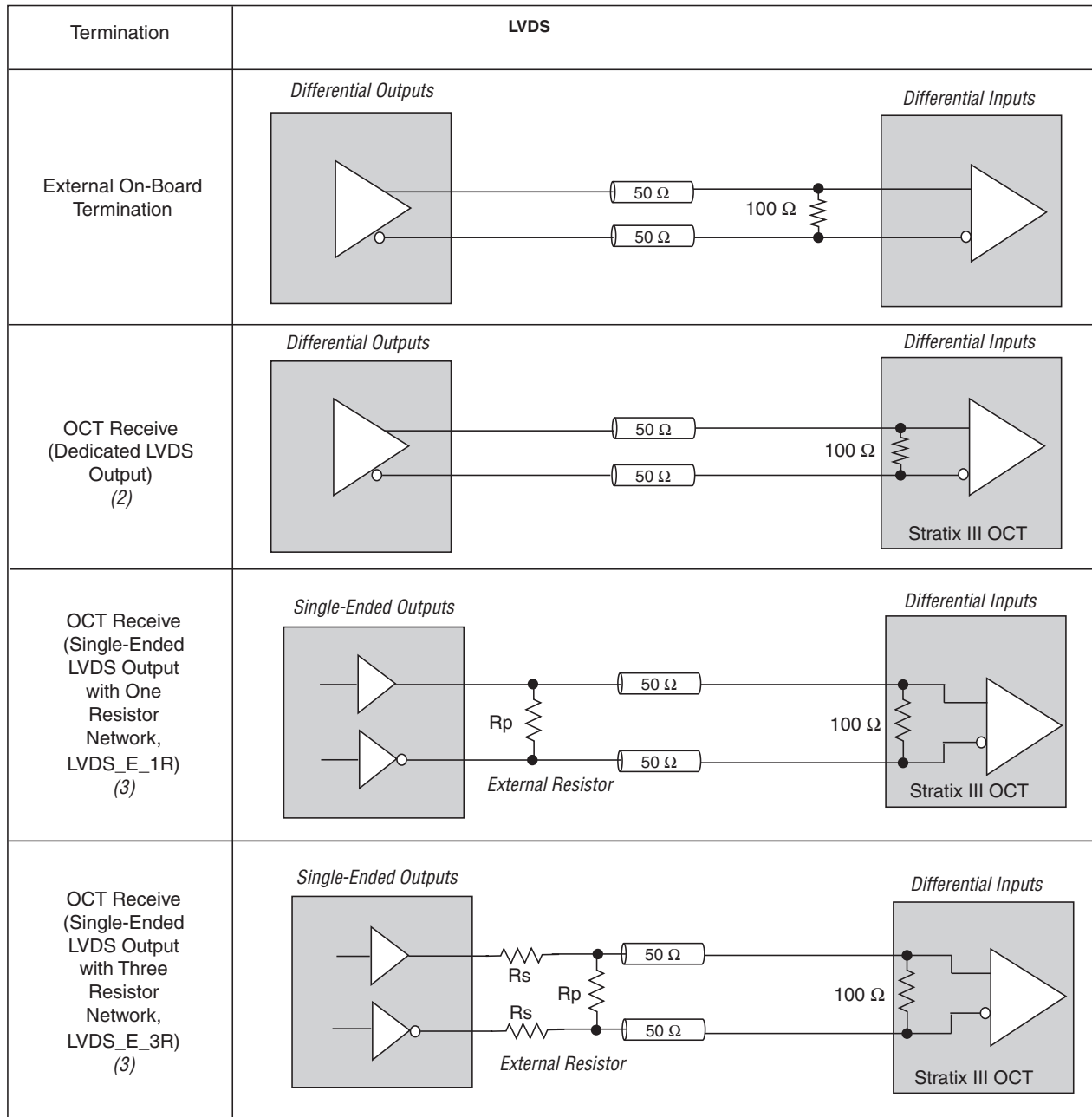
Figure 7–25. Stratix III LVDS I/O Standard Termination Note (1)
