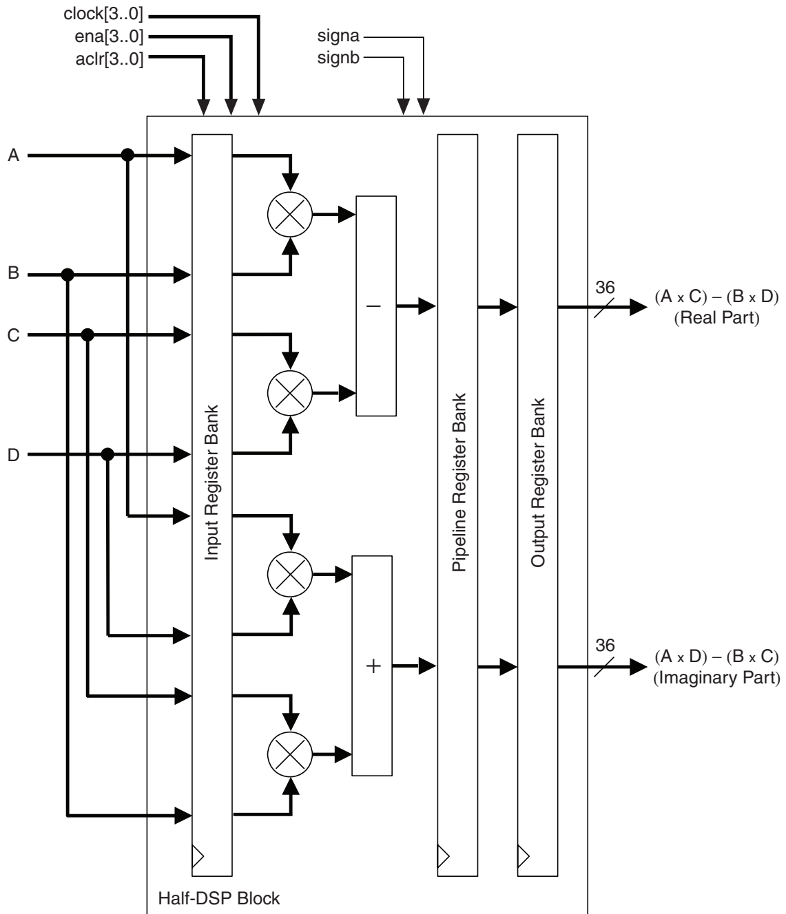
Figure 5–16. Complex Multiplier Using Two-Multiplier Adder Mode
