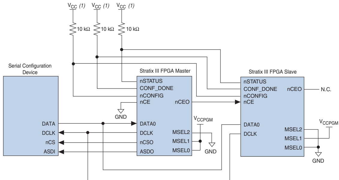
Figure 11–9. Multi-Device Fast AS Configuration
