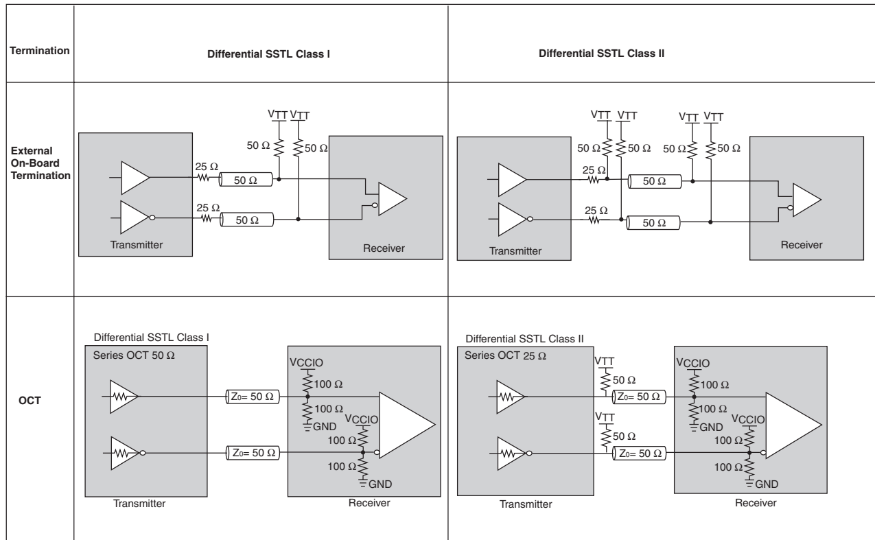
Figure 7–23. Stratix III Differential SSTL I/O Standard Termination
