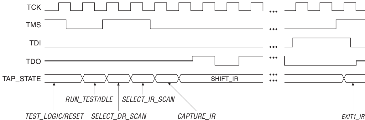
Figure 13–7. Selecting the Instruction Mode
