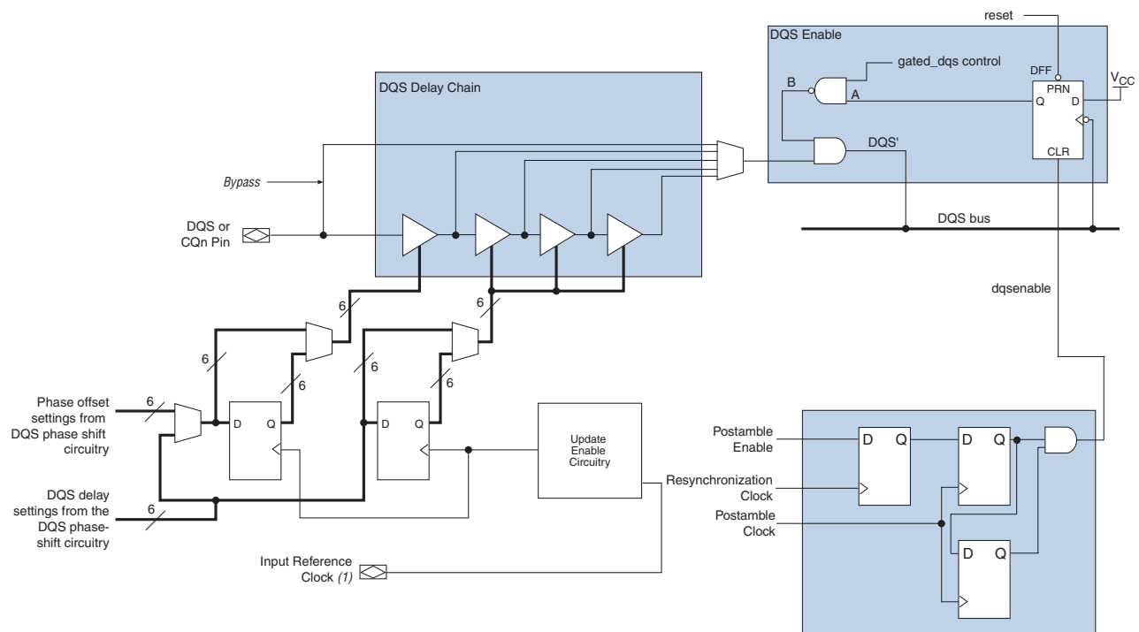
Figure 8–13. Stratix III DQS Logic Block
