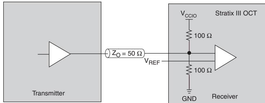
Figure 7–11. Stratix III On-Chip Parallel Termination with Calibration
