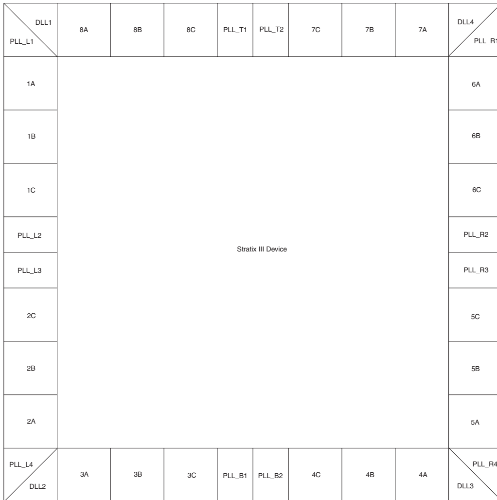
Figure 8–1. Stratix III Package Bottom View Note (1), (2)
