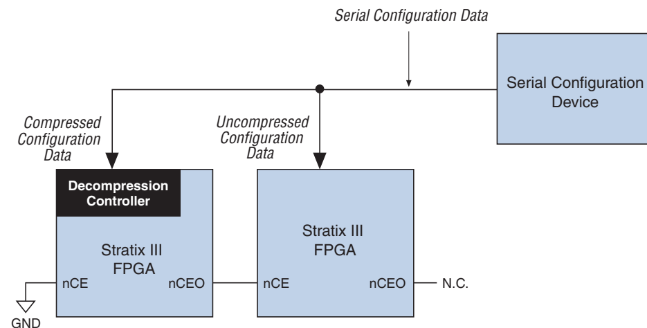
Figure 11–2. Compressed and Uncompressed Configuration Data in the Same Configuration File
