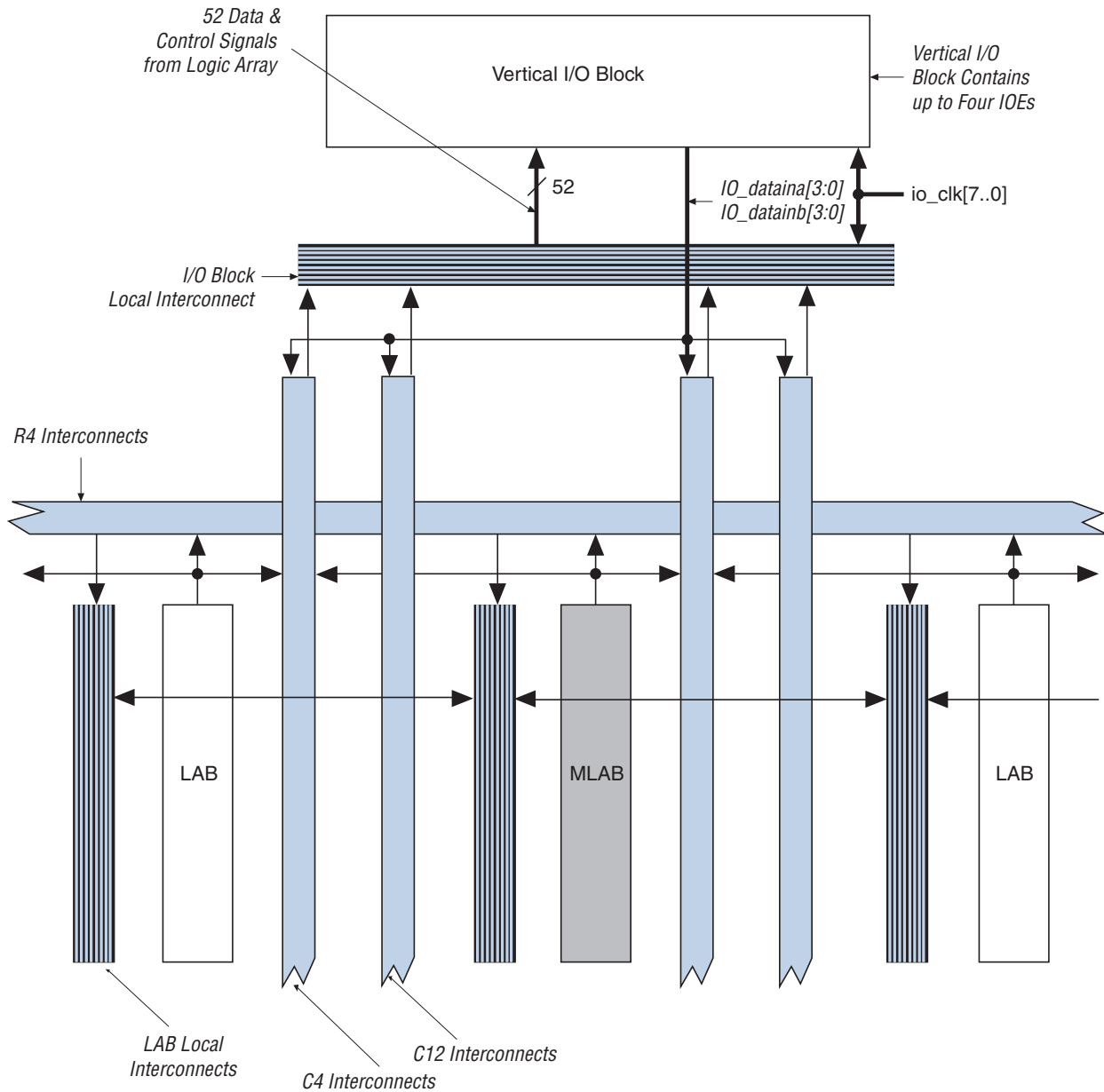
Figure 3–10. Column I/O Block Connection to Interconnect
