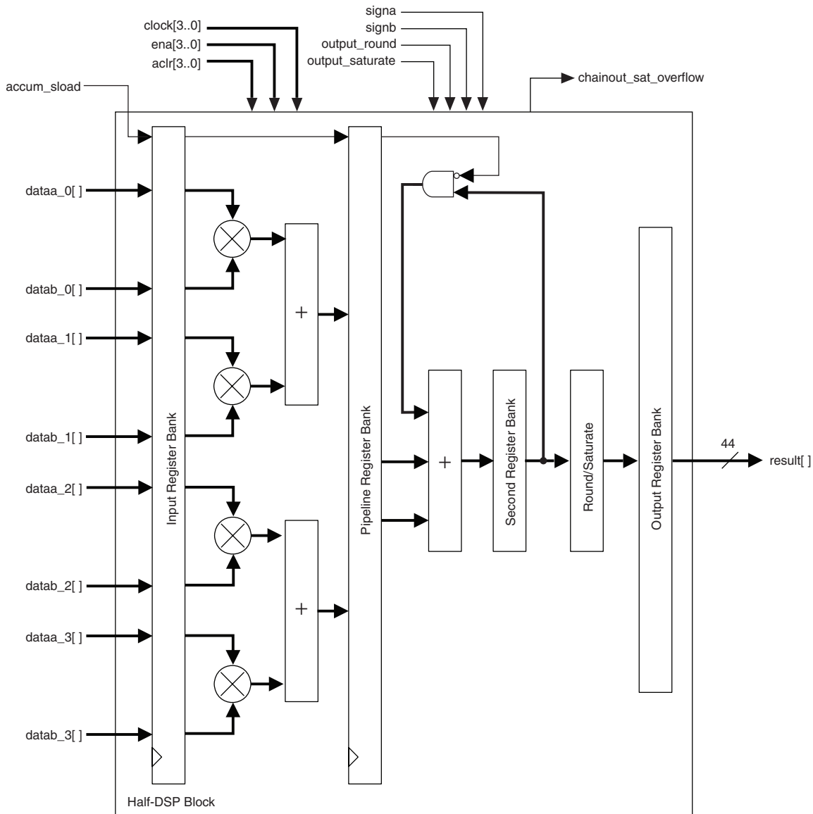
Figure 5-18. Multiply Accumulate Mode Shown for Half-DSP Block
