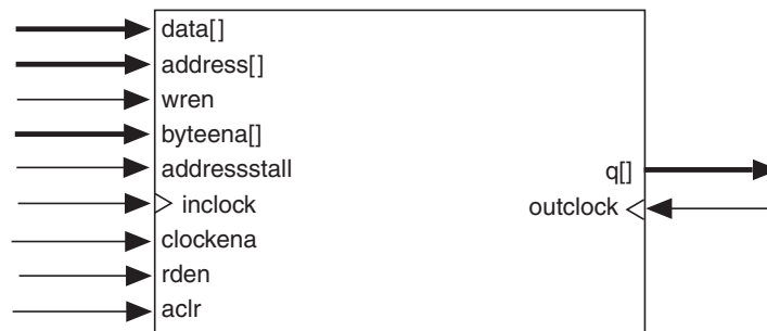
Figure 4–7. Single-Port Memory Note (1)
