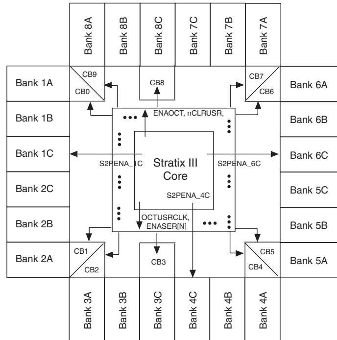
Figure 7–18. Signals Used for User Mode Calibration
