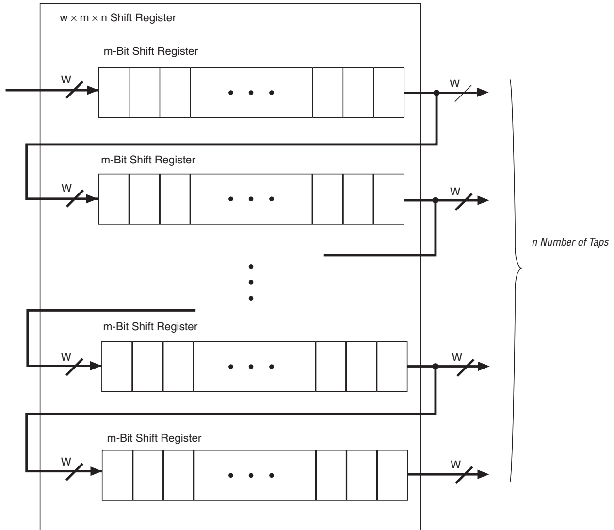
Figure 4–14. Stratix III Shift-Register Memory Configuration
