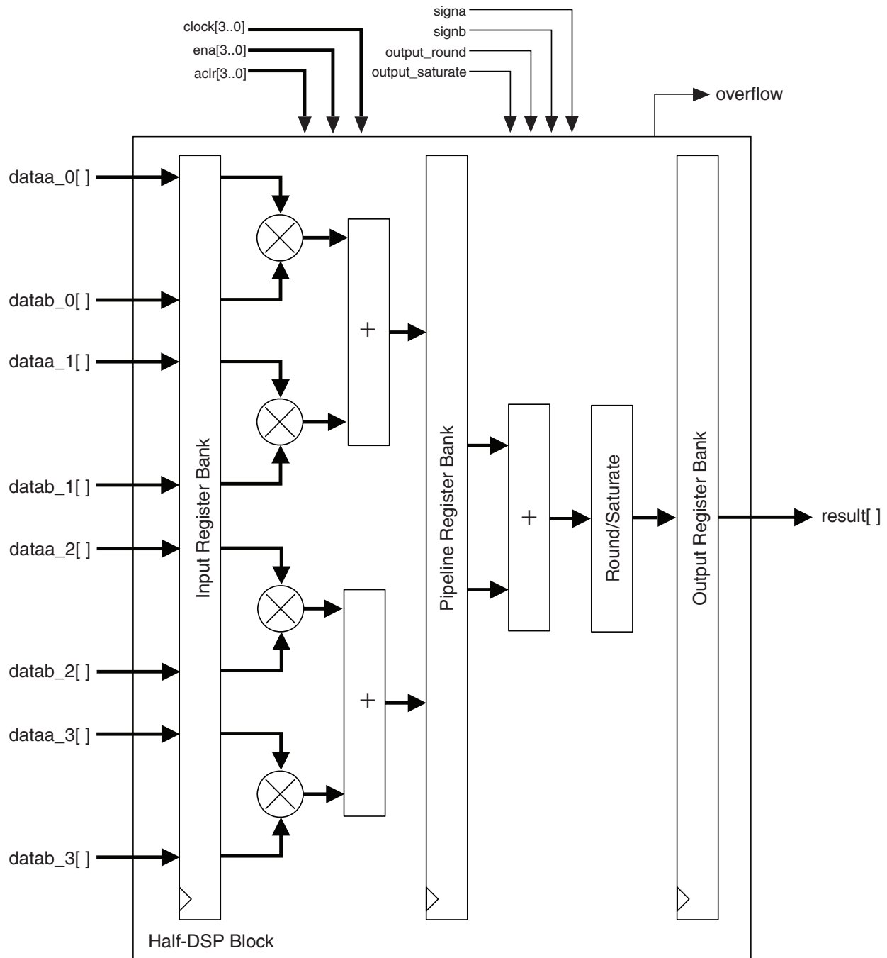
Figure 5–17. Four-Multiplier Adder Mode Shown for Half-DSP Block
