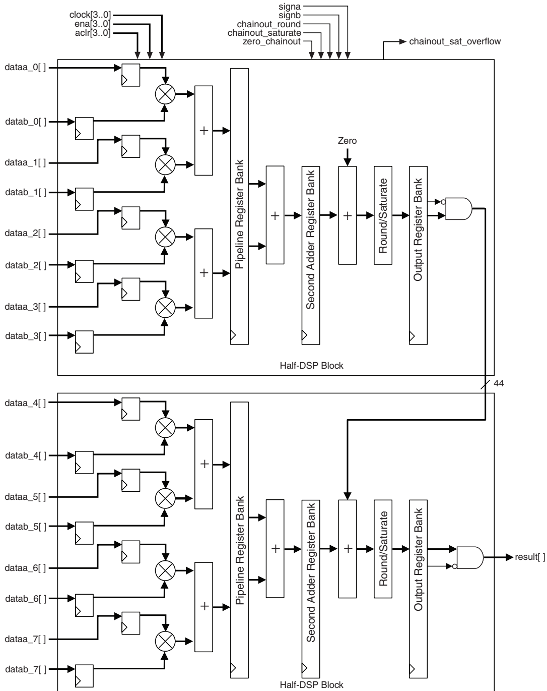
Figure 5–23. Semi-Parallel FIR Structure Using Chained Cascaded Summation
