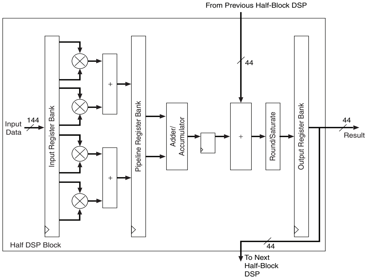
Figure 5–4. Output Cascading Feature for FIR Structures
