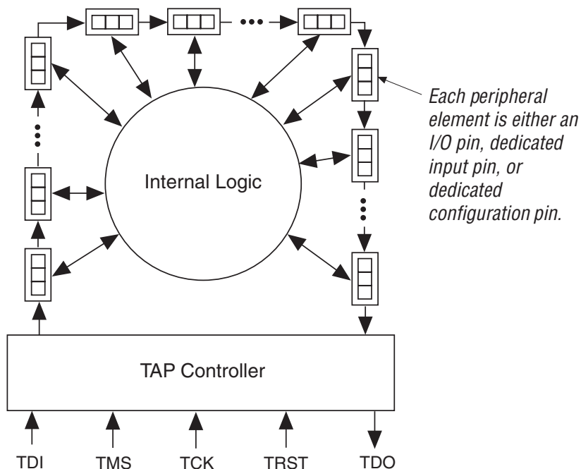
Figure 13–3. Boundary-Scan Register
