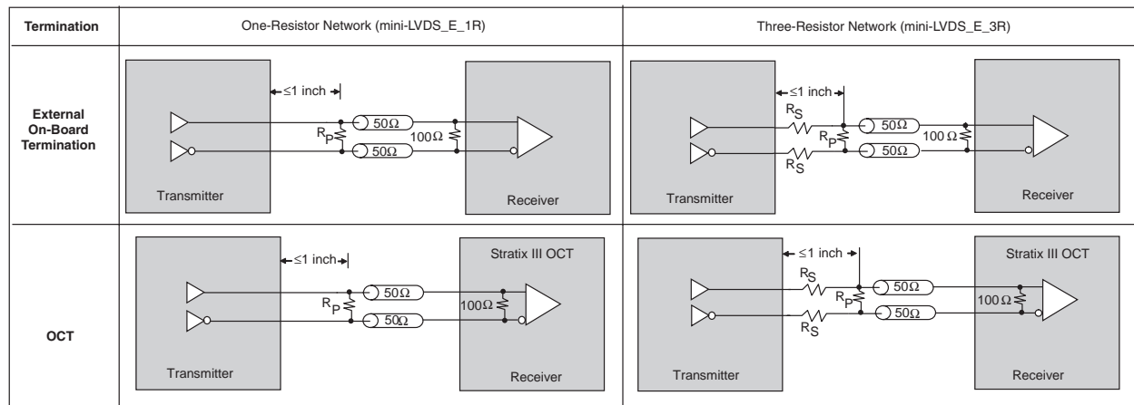
Figure 7–29. Stratix III mini-LVDS I/O Standard Termination Note (1)
