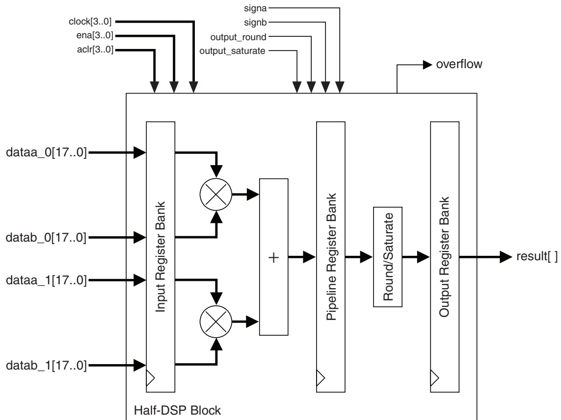
Figure 5–14. Two-Multiplier Adder Mode Shown for Half-DSP Block
