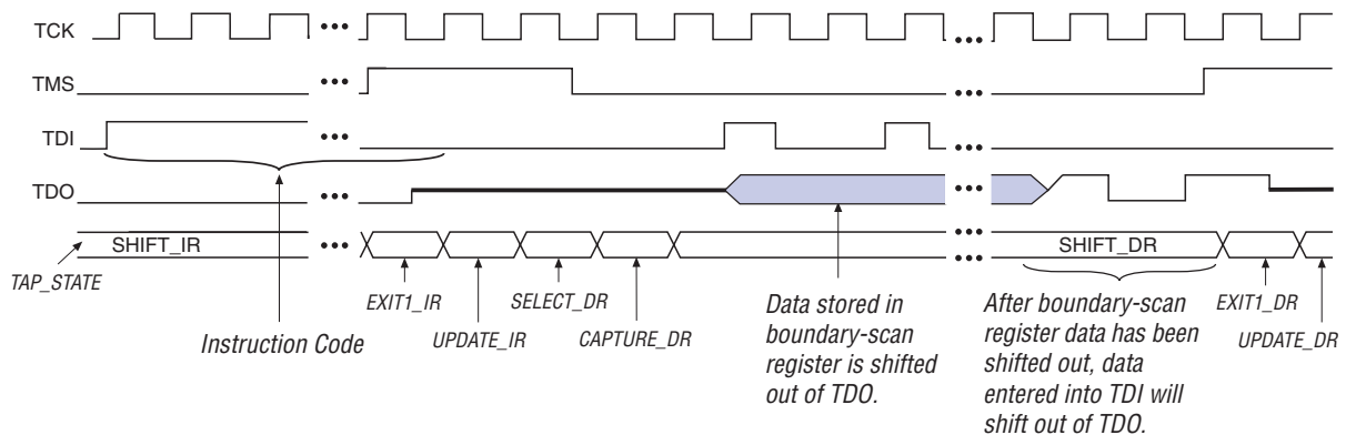
Figure 13–11. EXTEST Shift Data Register Waveforms
