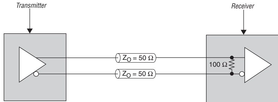
Figure 7–13. Differential Input On-Chip Termination
