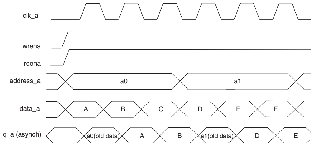
Figure 4-8. Timing Waveform for Read-Write Operations (Single-Port Mode)
