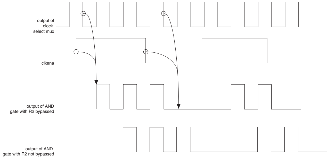
Figure 6–15. clkena Signals
