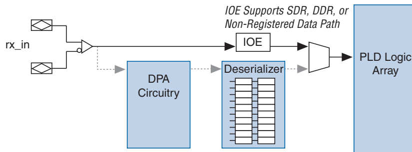
Figure 9–6. Stratix III Deserializer Bypass
