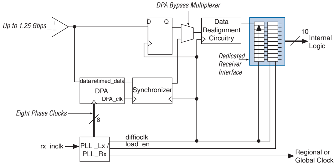
Figure 9–5. Receiver Block Diagram
