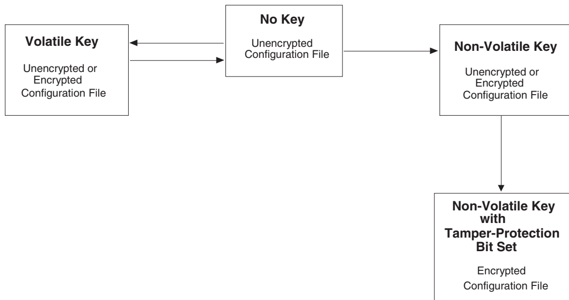
Figure 14–2. Stratix III Security Modes - Sequence and Restrictions
