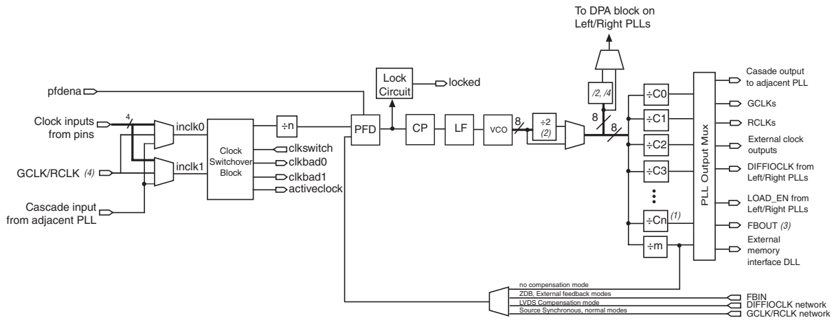
Figure 6–17. Stratix III PLL Block Diagram
