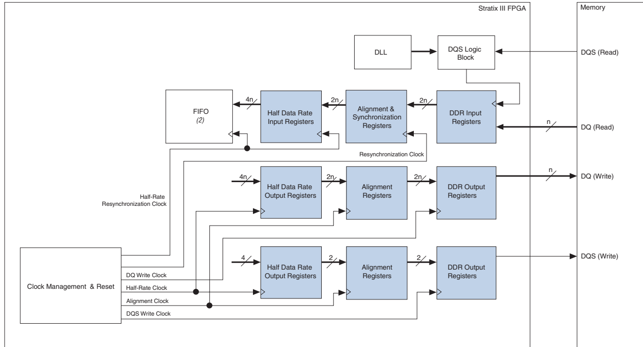
Figure 8–2. External Memory Interface Data Path Overview Note (1), (2)
