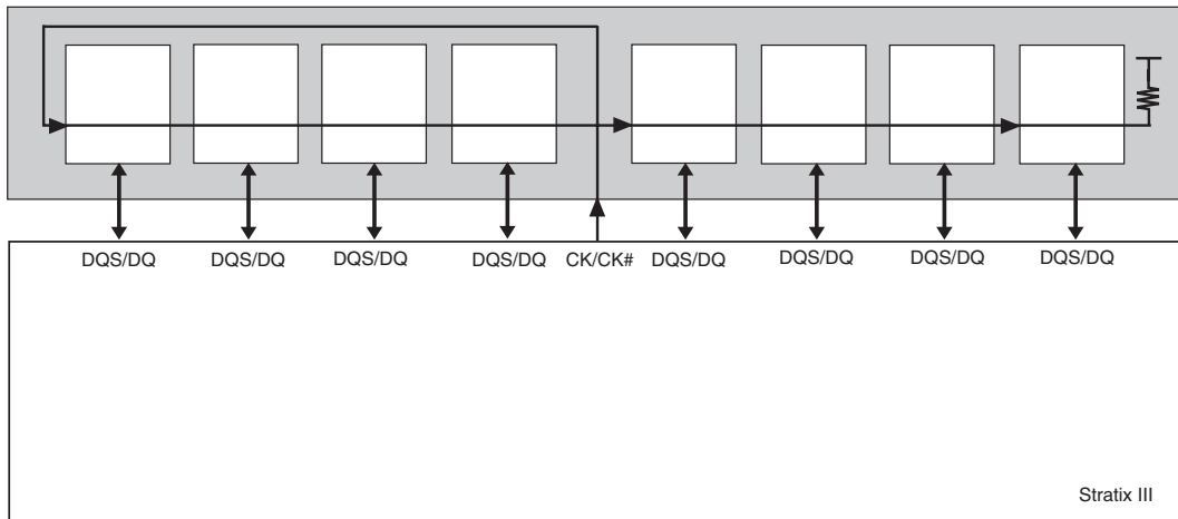
Figure 8–17. DDR3 SDRAM Unbuffered Module Clock Topology
