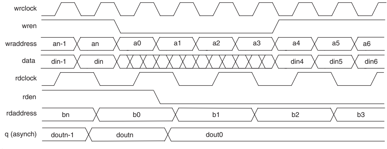
Figure 4–10. Stratix III Simple Dual-Port Timing Waveforms
