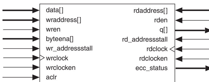
Figure 4–9. Stratix III Simple Dual-Port Memory Note (1)
