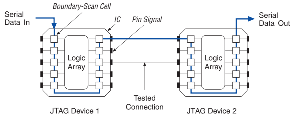
Figure 13–1. IEEE Std. 1149.1 Boundary-Scan Testing
