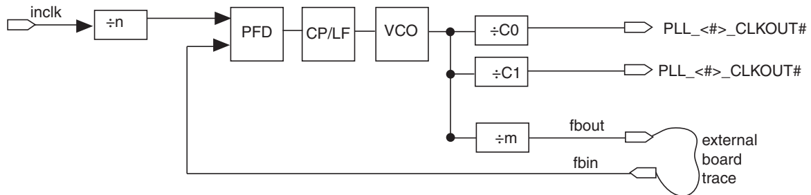
Figure 6–26. External Feedback Mode in Stratix III Devices
