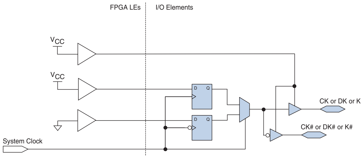
Figure 8-9. Memory Clock Generation Block Diagram Note (1), (2)
