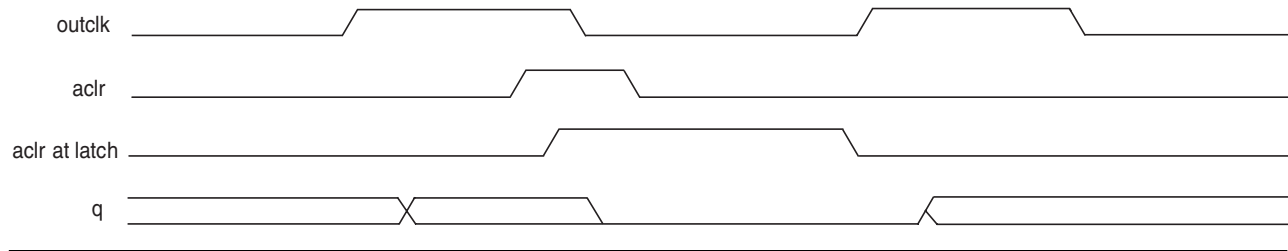
Figure 4–5. Output Latch Asynchronous Clear Waveform
