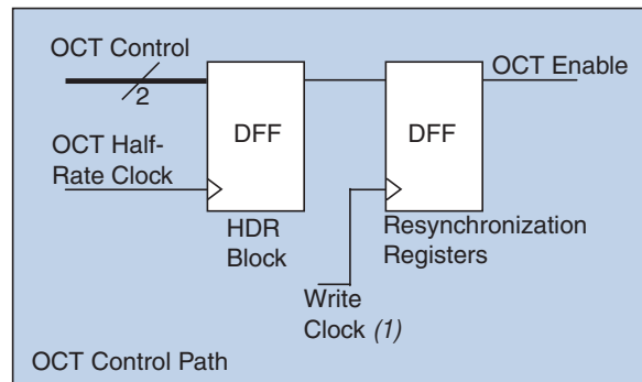
Figure 8–19. Stratix III Dynamic OCT Control Block
