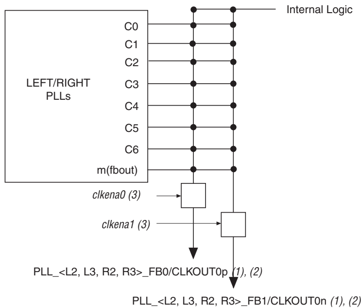
Figure 6–19. External Clock Outputs for Left/Right PLLs
