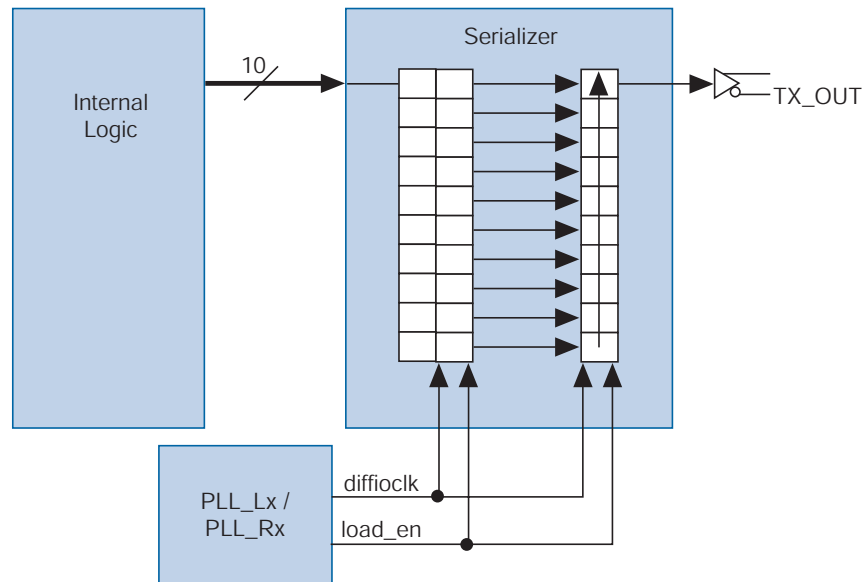
Figure 9–2. Stratix III Transmitter Block Diagram
