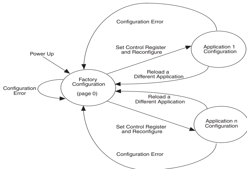
Figure 12–4. Transitions Between Configurations in Remote Update Mode
