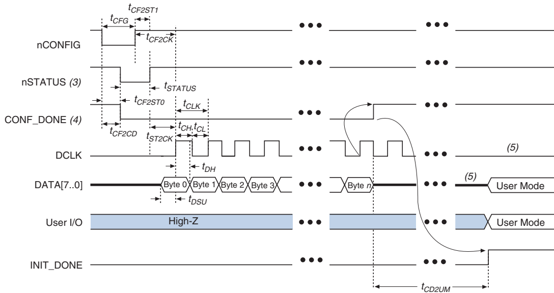
Figure 11–6. FPP Configuration Timing Waveform Notes (1), (2)
