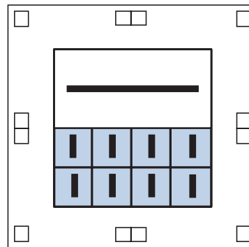
Figure 6-7. Eight Independent Sub-Regional + One Dual-Regional Clock Region
