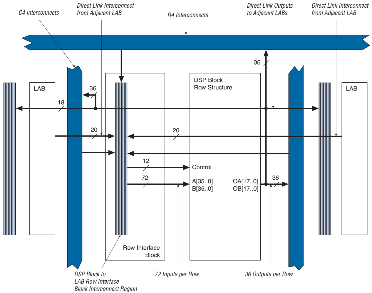
Figure 3–8. Detailed View, DSP Block Interface to Interconnect
