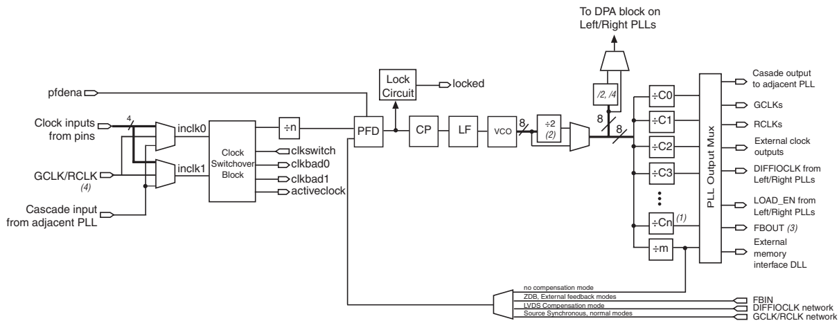
Figure 9–12. PLL Block Diagram
