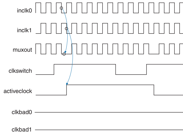
Figure 6–31. Clock Switchover Using the clkswitch (Manual) Control
