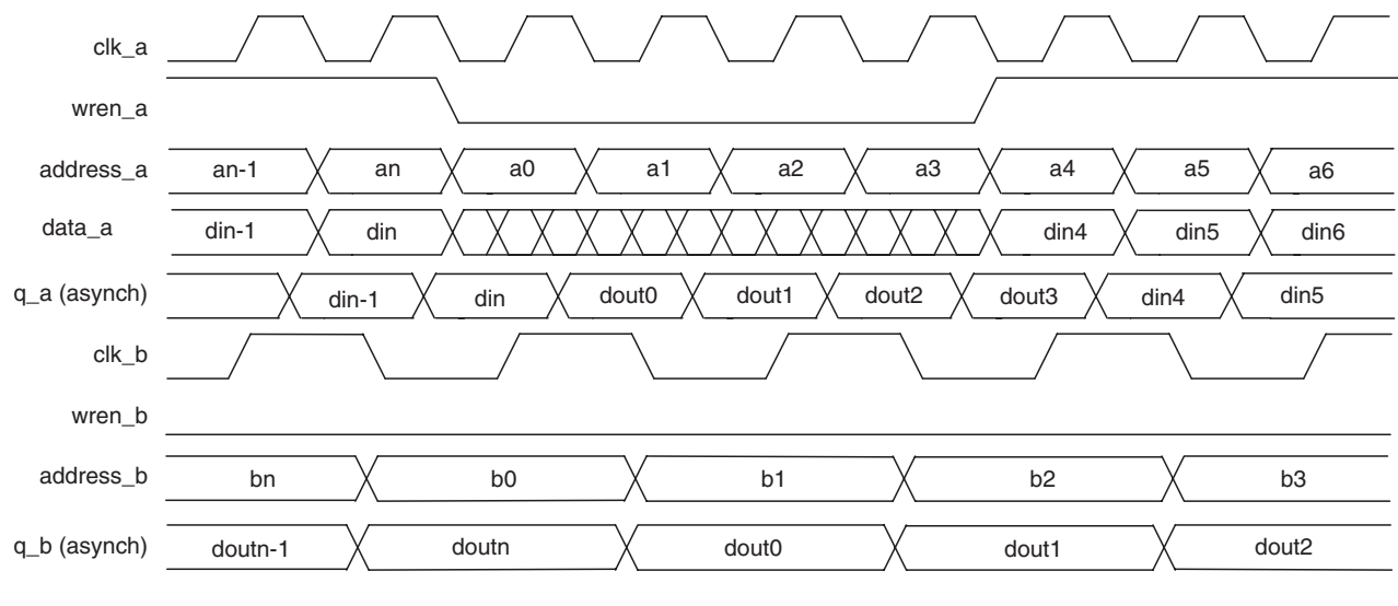
Figure 4–13. Stratix III True Dual-Port Timing Waveform
