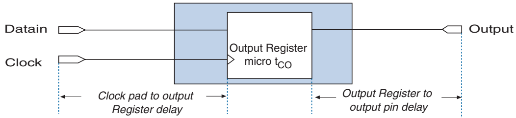
Figure 1–3. Output Register Clock to Output Timing Diagram
