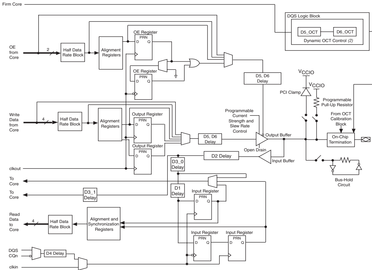
Figure 7–8. Stratix III IOE Structure Notes (1), (2)
