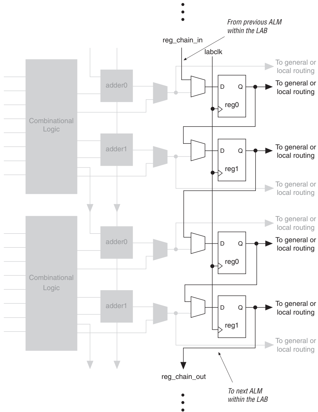
Figure 2–17. Register Chain within an LAB Note (1)
