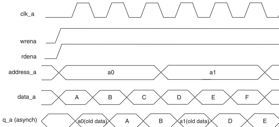
Figure 4–17. Same Port Read-During-Write: Old Data Mode
