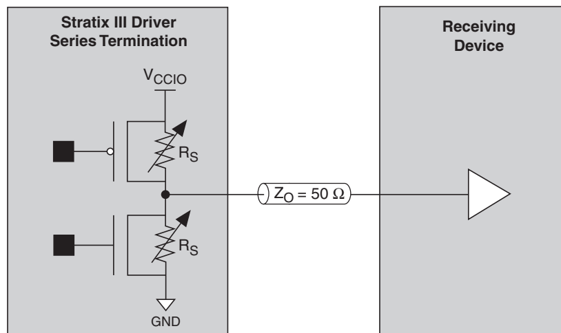
Figure 7-10. Stratix III On-Chip Series Termination with Calibration
