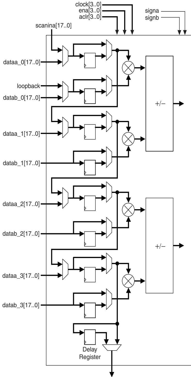
Figure 5–7. Input Register of Half-DSP Block
