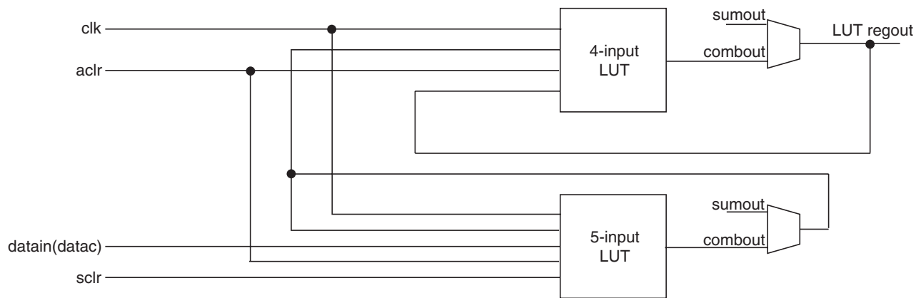
Figure 2–15. LUT Register from Two Combinational Blocks
