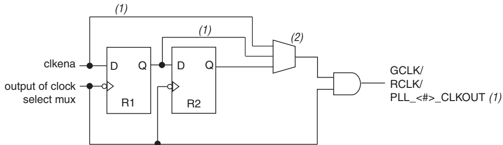
Figure 6–14. ckena Implementation
