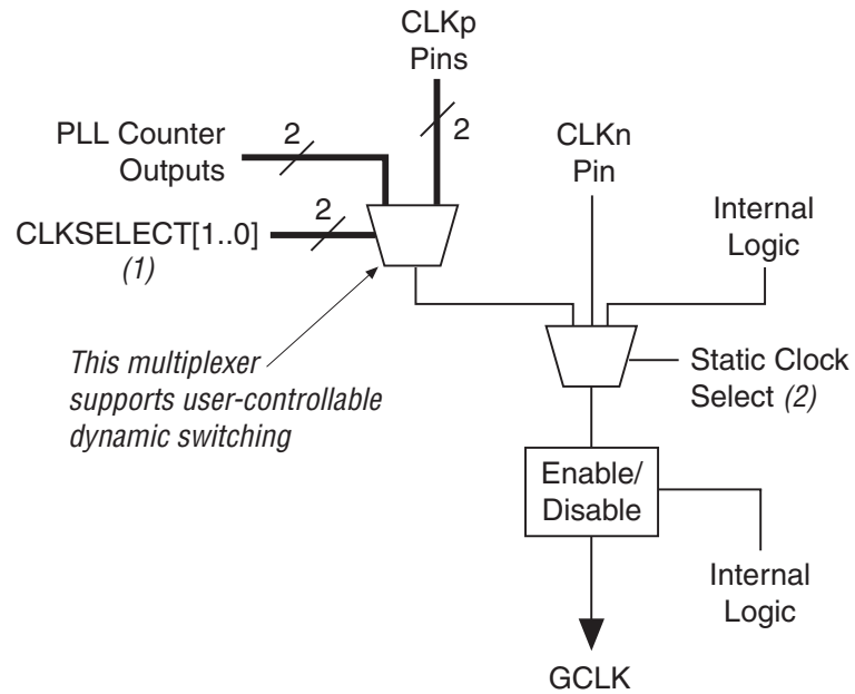
Figure 6–11. Stratix III Global Clock Control Block
