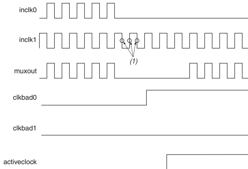
Figure 6–30. Automatic Switchover Upon Loss of Clock Detection
