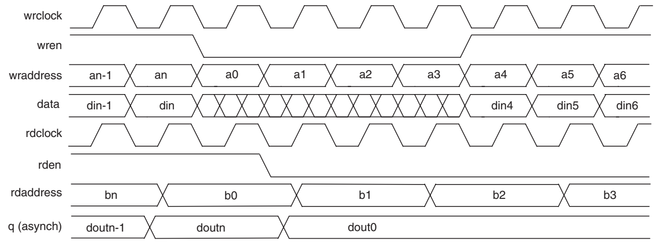
Figure 4–11. Stratix III Mixed-Port Read-During-Write Timing Waveforms
