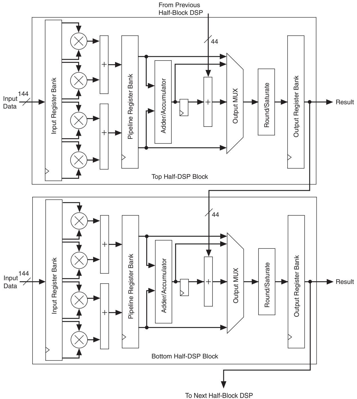
Figure 5-5. Stratix III Full DSP Block Summary
