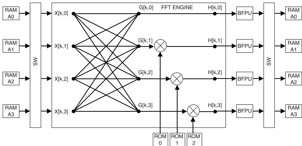
Figure 5–24. Radix-4 Butterfly
