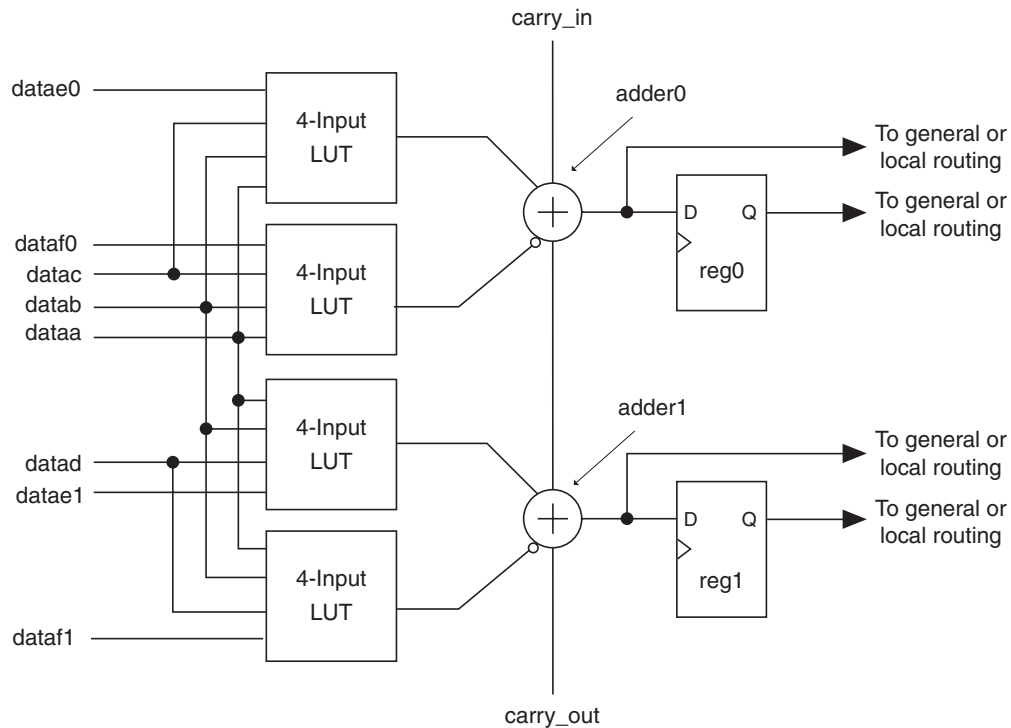
Figure 2–11. ALM in Arithmetic Mode
