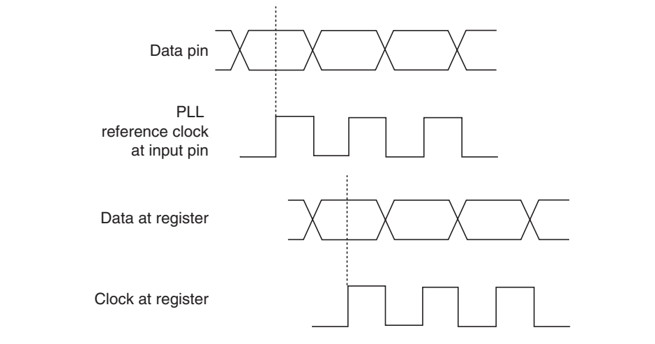
Figure 6–21. Phase Relationship Between Clock and Data in Source-Synchronous and LVDS Modes
