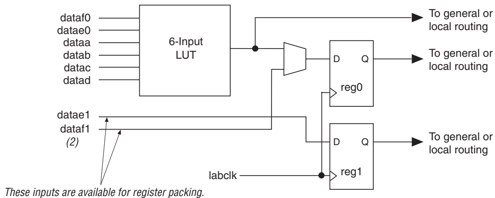
Figure 2–9. Input Function in Normal Mode Note (1)
