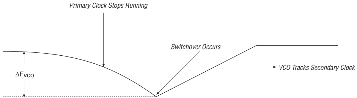
Figure 6–33. VCO Switchover Operating Frequency
