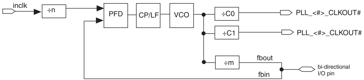
Figure 6–24. Zero-Delay Buffer Mode in Stratix III PLLs
