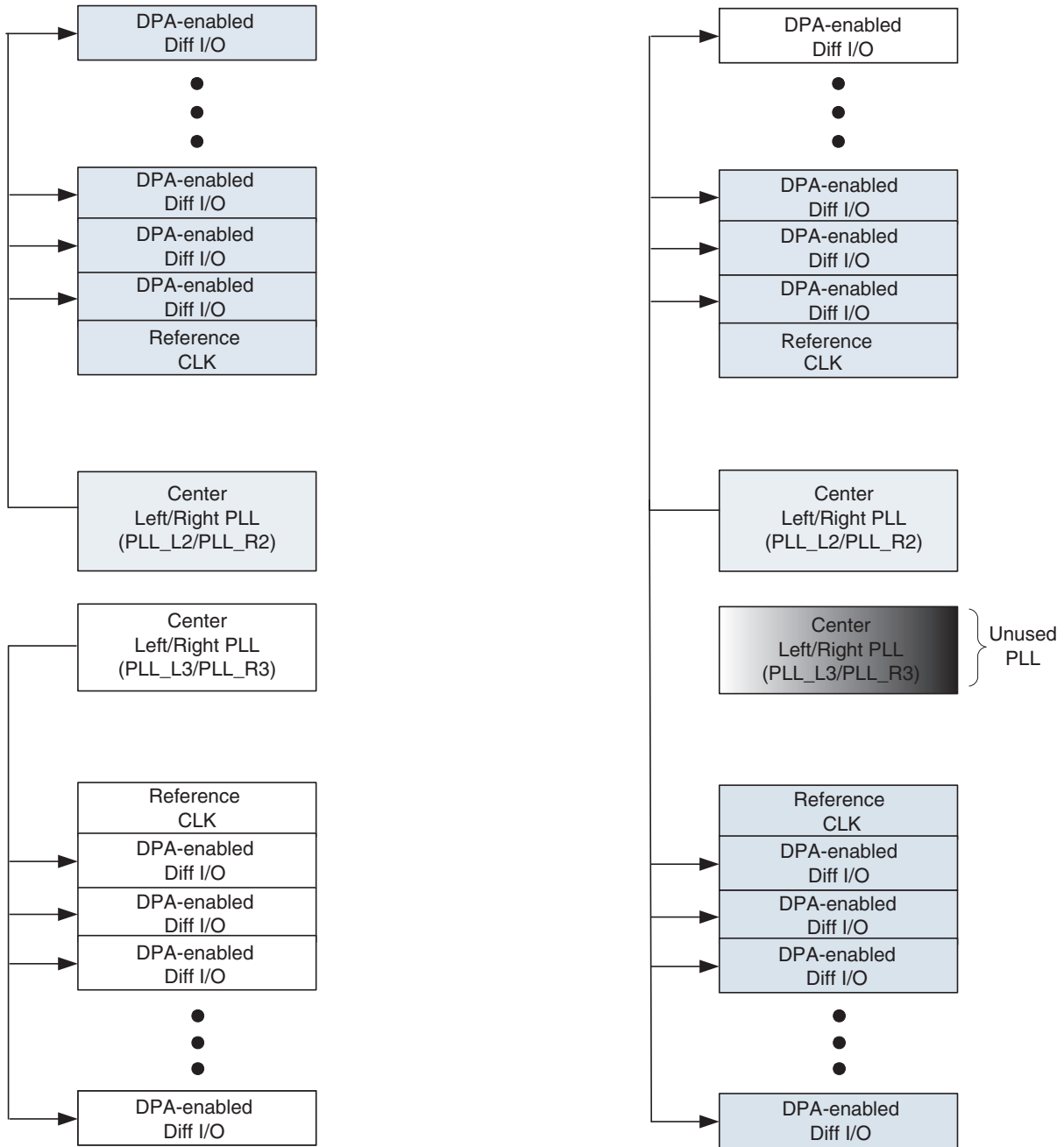
Figure 9–21. Center Left/Right PLLs Driving DPA-Enabled Differential I/Os
