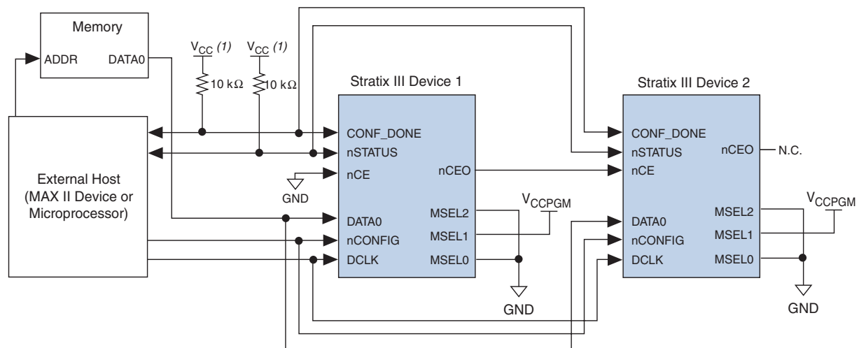
Figure 11–14. Multi-Device PS Configuration Using an External Host
