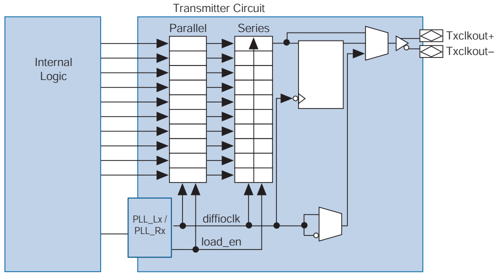
Figure 9–3. Stratix III Transmitter in Clock Output Mode
