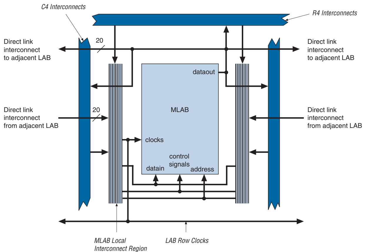
Figure 3–4. MLAB RAM Block LAB Row Interface
