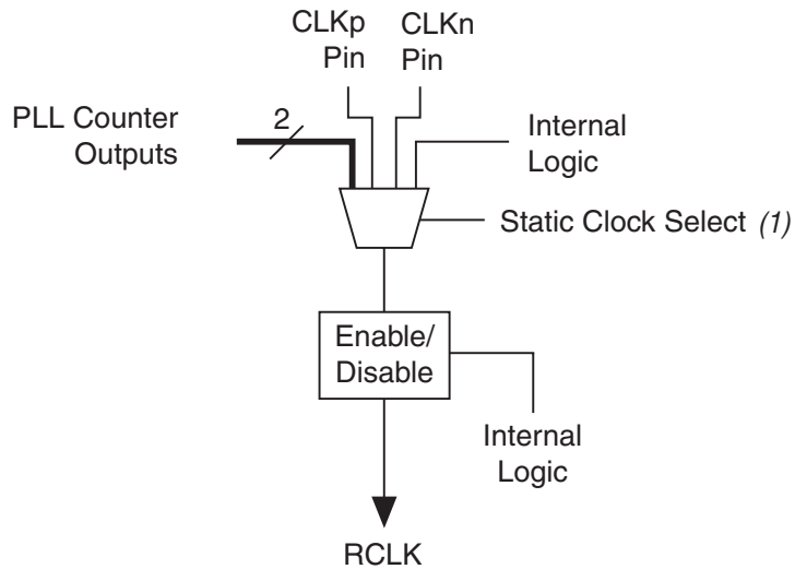
Figure 6–12. Regional Clock Control Block
