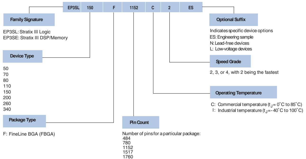
Figure 1–1. Stratix III Device Packaging Ordering Information
