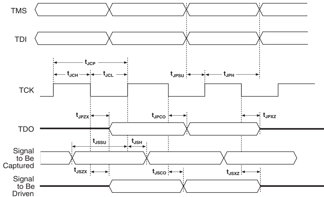
Figure 13–6. IEEE Std. 1149.1 Timing Waveforms
