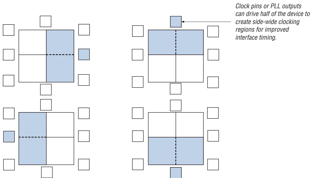
Figure 6-5. Stratix III Dual-Regional Clock Region
