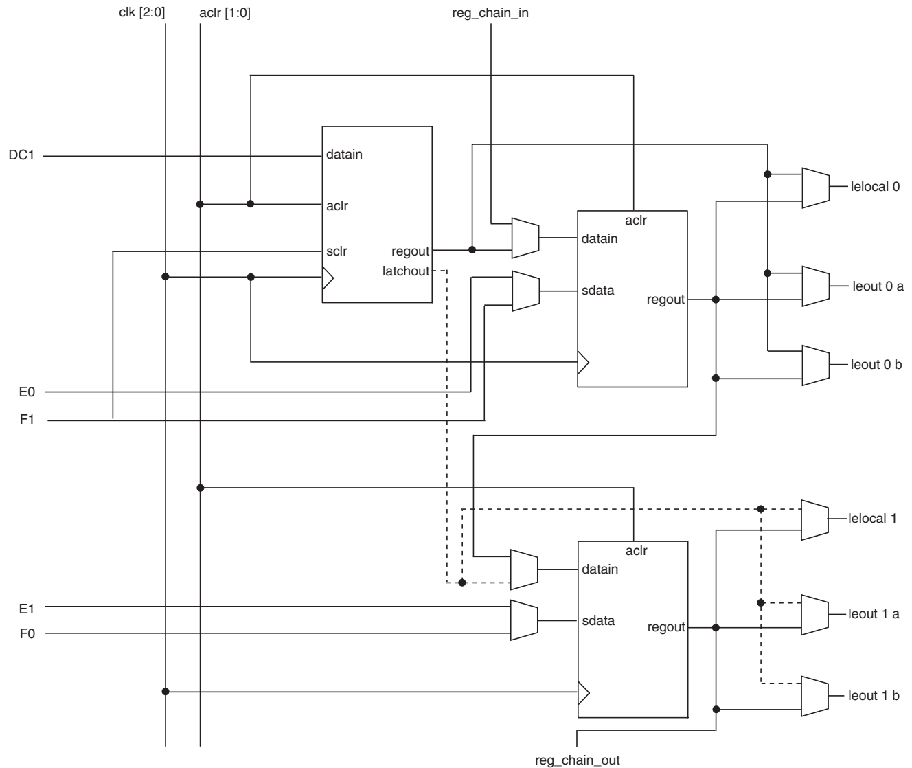
Figure 2–16. ALM in LUT-Register Mode with 3-Register Capability
