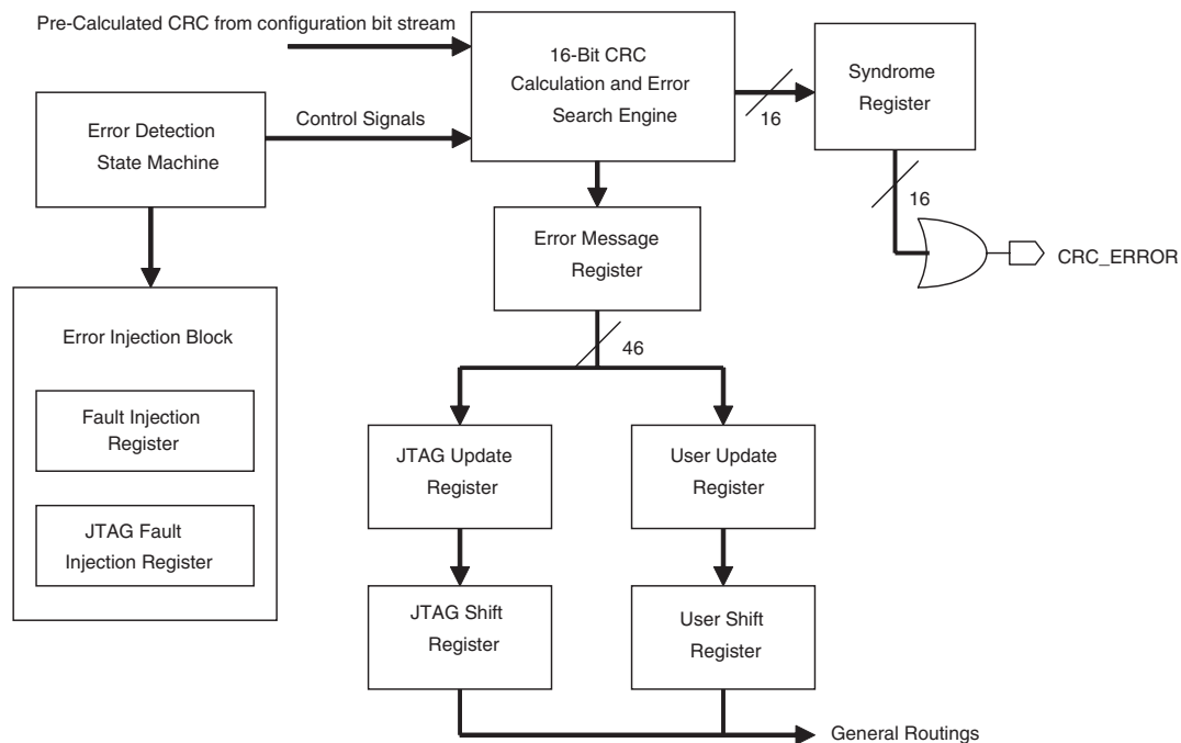
Figure 15–2. Error Detection Block Diagram
