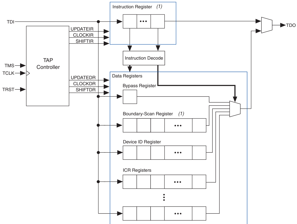
Figure 13–2. IEEE Std. 1149.1 Circuitry
