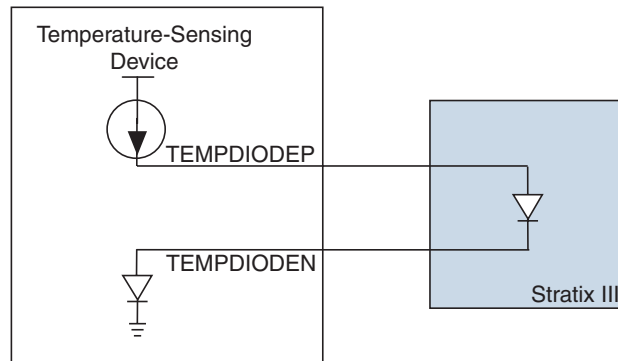
Figure 16–2. TSD Connections
