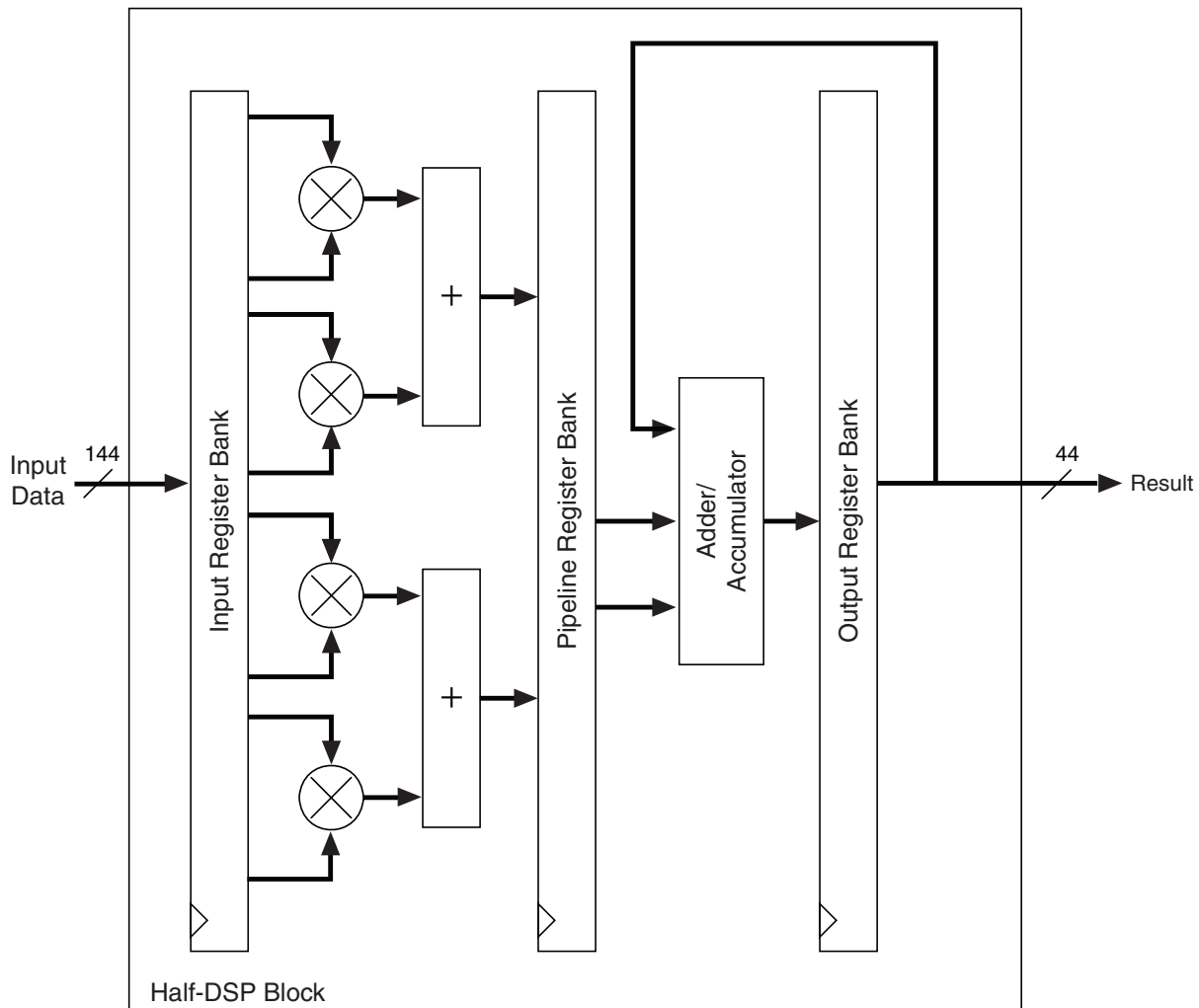
Figure 5–3. Four-Multiplier Adder and Accumulation Capability
