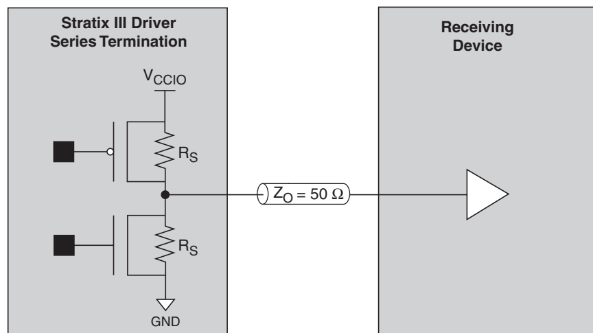
Figure 7-9. Stratix III On-Chip Series Termination without Calibration
