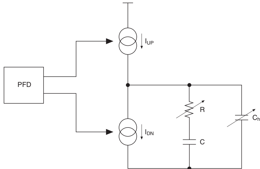
Figure 6–35. Loop Filter Programmable Components
