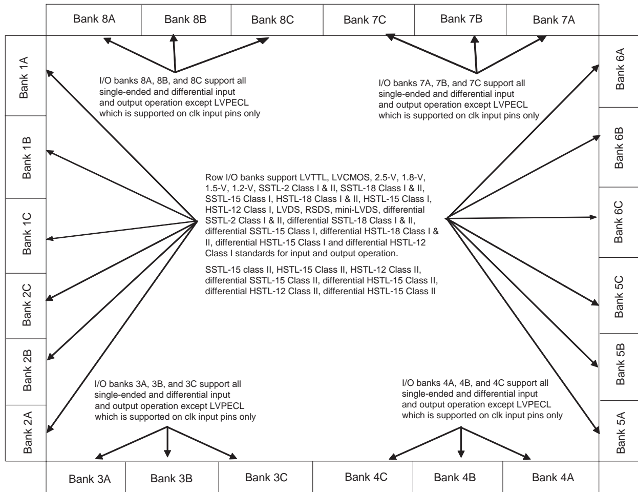
Figure 7–1. Stratix III I/O banks Notes (1), (2), (3), (4), (5), (6), (7), (8), (9)
