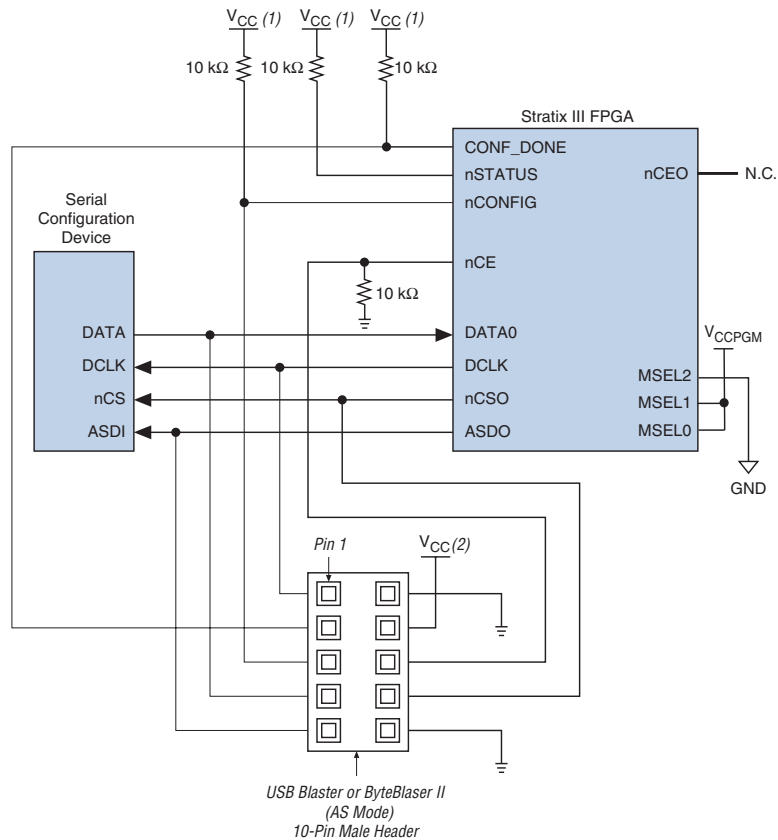
Figure 11–11. In-System Programming of Serial Configuration Devices
