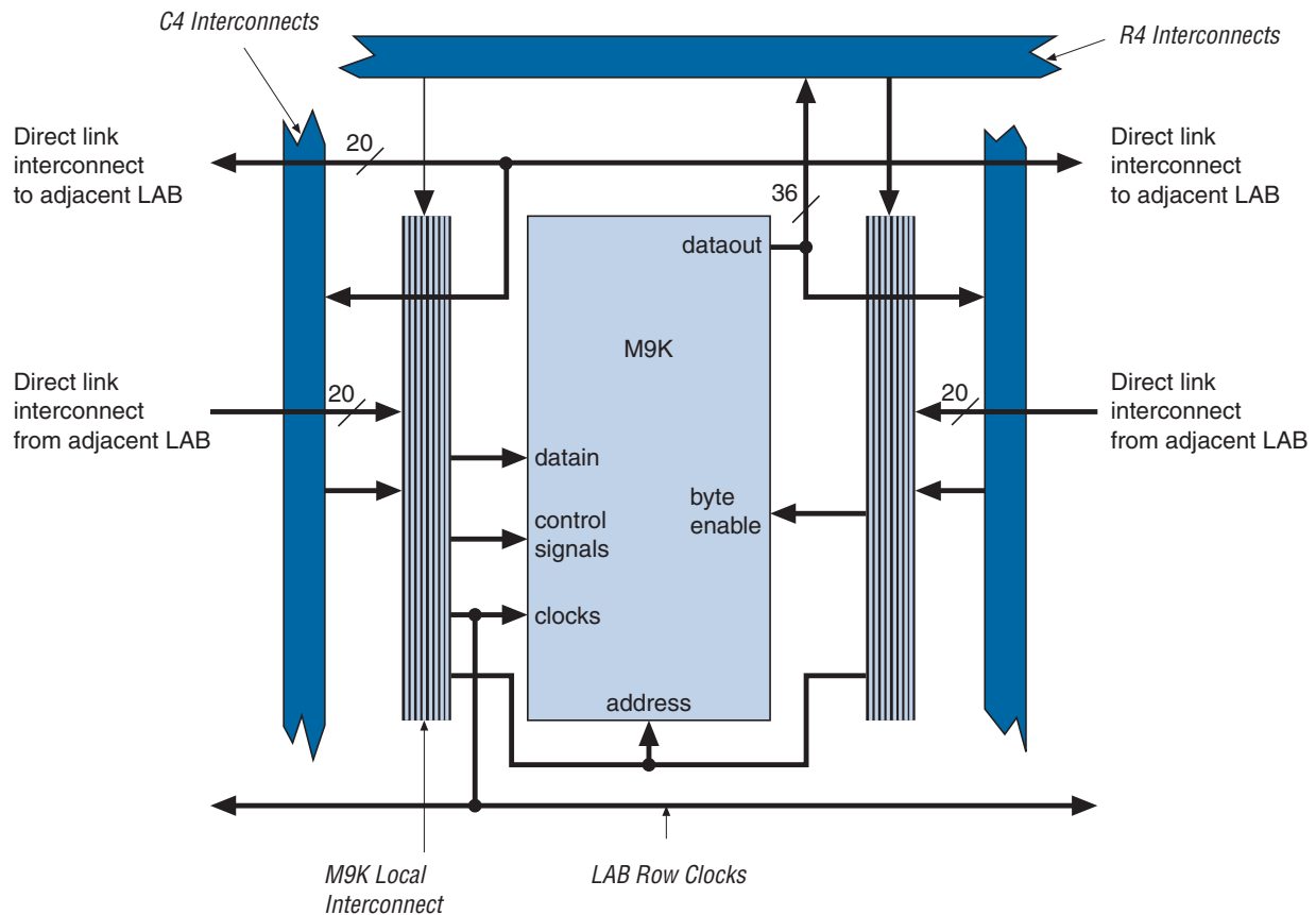
Figure 3–5. M9K RAM Block LAB Row Interface
