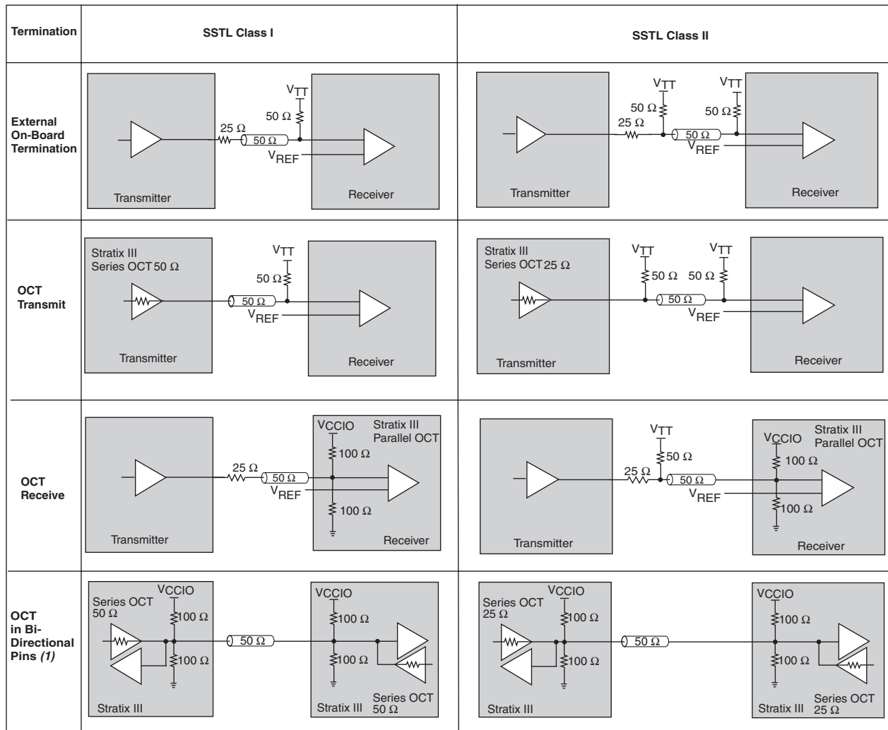
Figure 7–21. Stratix III SSTL I/O Standard Termination
