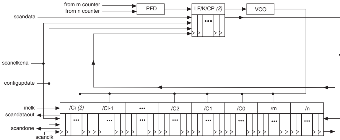
Figure 6–37. PLL Reconfiguration Scan Chain
