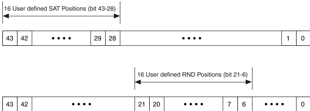
Figure 5–20. Round and Saturation Locations
