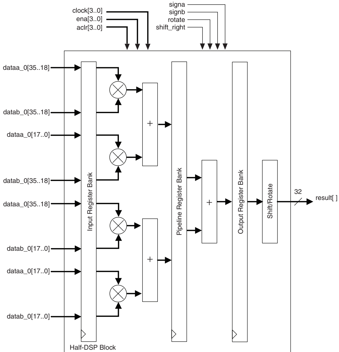
Figure 5-19. Shift Operation Mode Shown for Half-DSP Block
