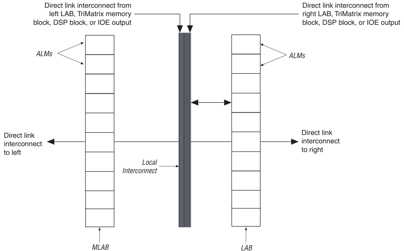
Figure 2-3. Direct Link Connection
