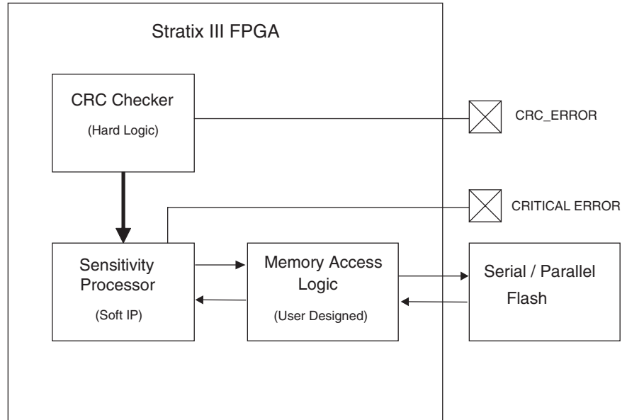
Figure 15–1. Critical Error Detection Implementation Block Diagram
