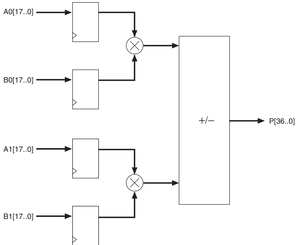
Figure 5–2. Basic Two-Multiplier Adder Building Block
