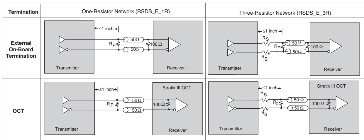
Figure 7–28. Stratix III RSDS I/O Standard Termination Note (1)
