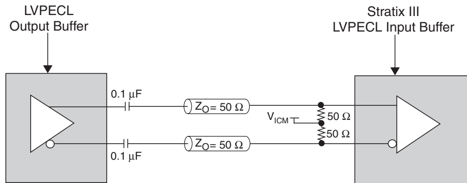
Figure 7–26. LVPECL AC Coupled Termination
