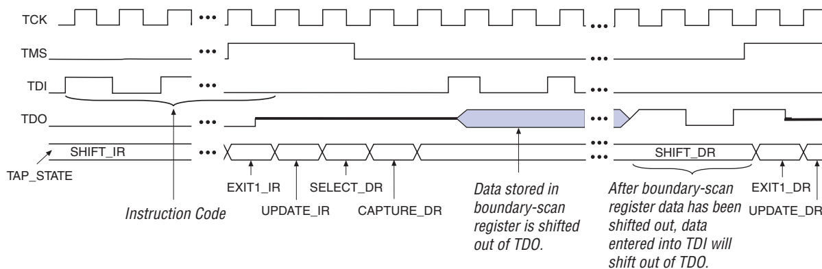
Figure 13–9. SAMPLE/PRELOAD Shift Data Register Waveforms
