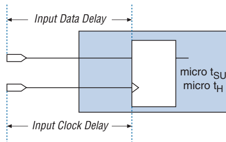
Figure 1–2. Input Register Setup and Hold Timing Diagram
