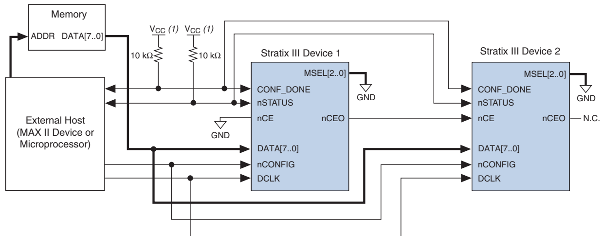
Figure 11–4. Multi-Device FPP Configuration Using an External Host
