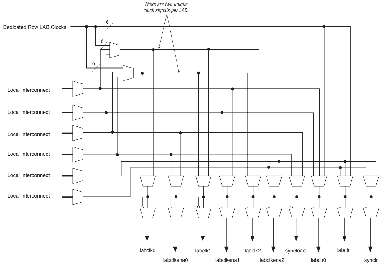
Figure 2-4. LAB-Wide Control Signals
