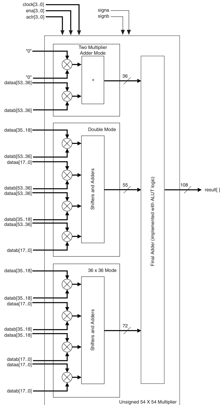
Figure 5–13. Unsigned 54 × 54 Multiplier
