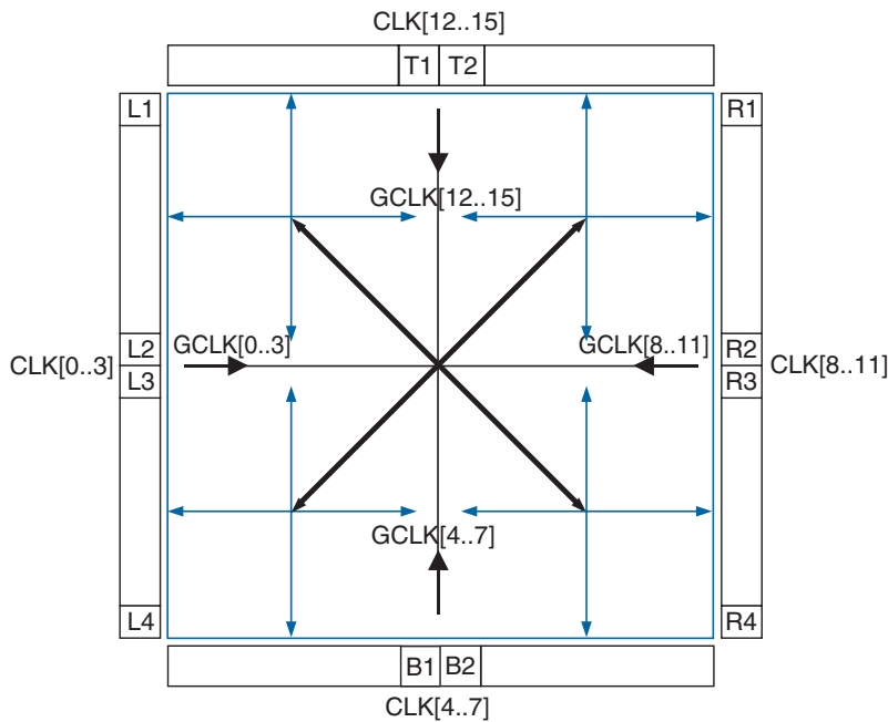
Figure 6–1. Global Clock Networks
