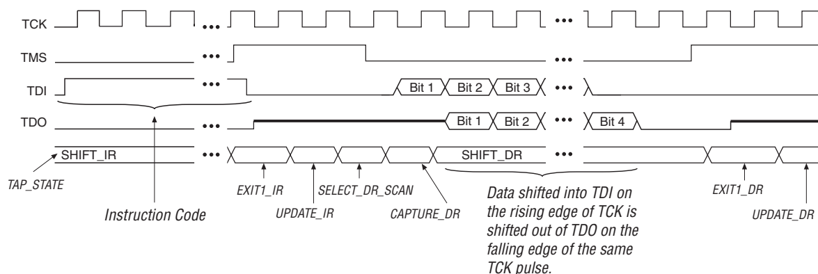
Figure 13–12. BYPASS Shift Data Register Waveforms
