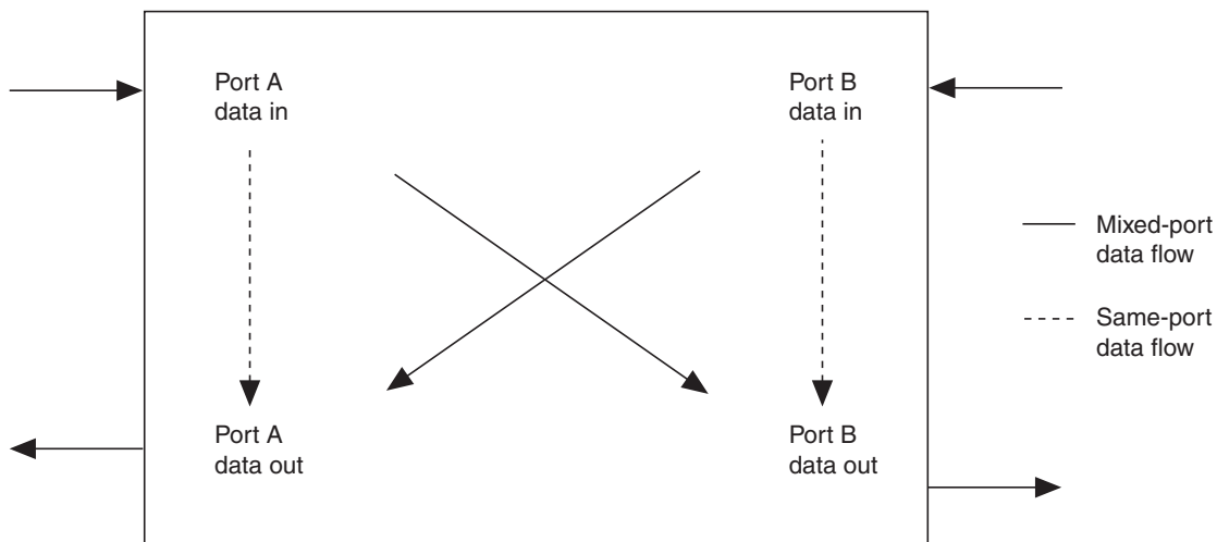
Figure 4–15. Stratix III Read-During-Write Data Flow
