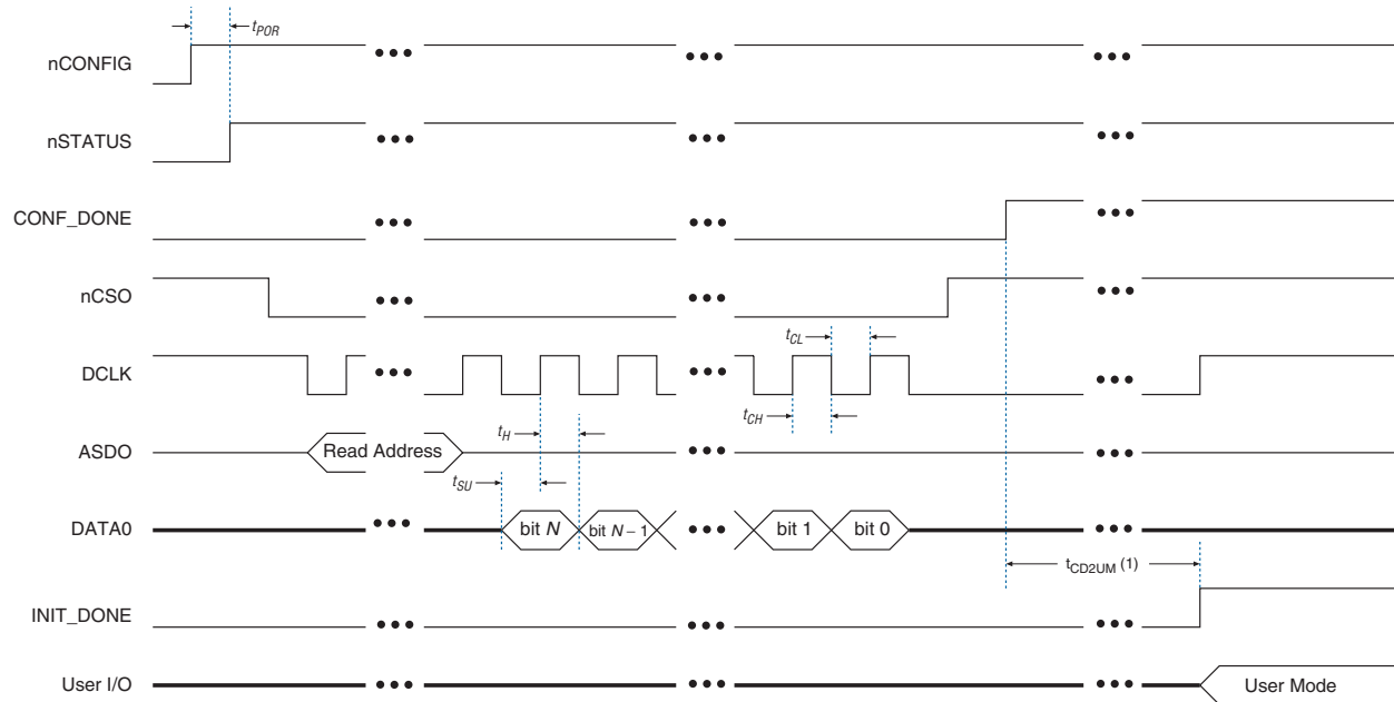
Figure 11–12. Fast AS Configuration Timing
