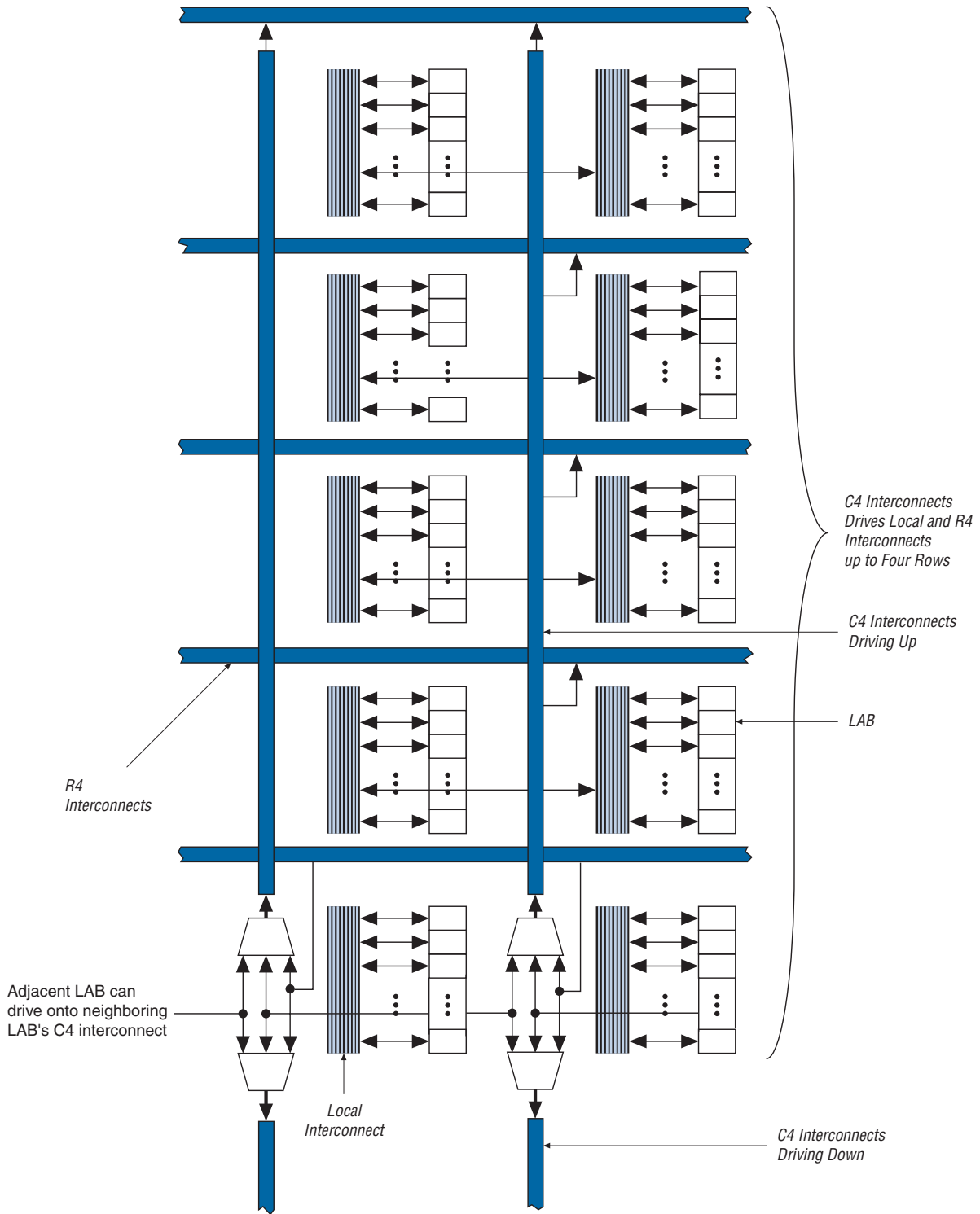
Figure 3-3. C4 Interconnect Connections Note (1)
