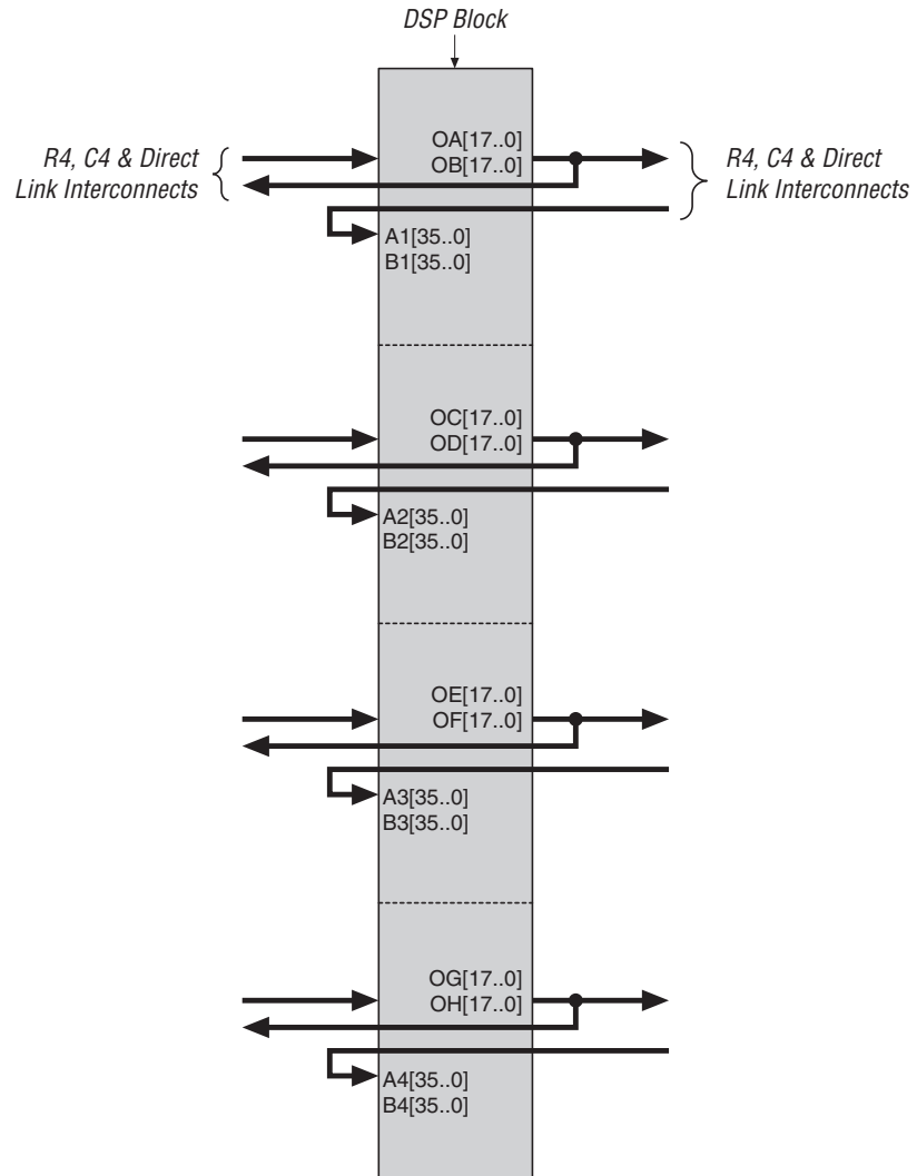
Figure 3-7. High-Level View, DSP Block Interface to Interconnect
