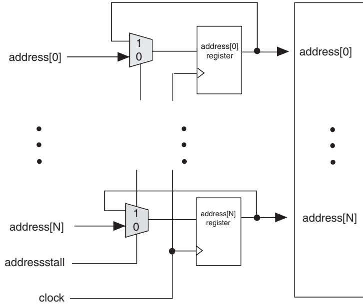
Figure 4–2. Stratix III Address Clock Enable Block Diagram
