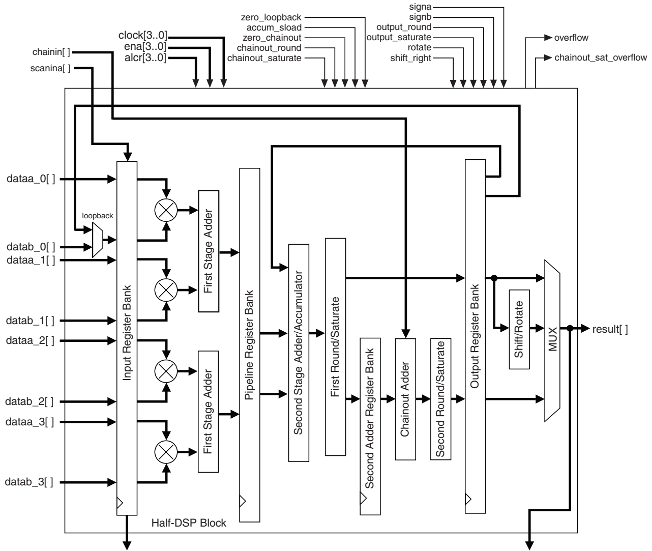
Figure 5–6. Half-DSP Block Architecture
