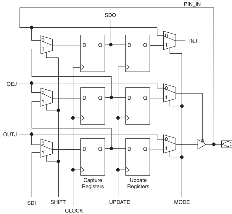
Figure 13–8. IEEE Std. 1149.1 BST SAMPLE/PRELOAD Mode
