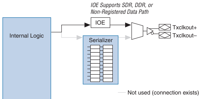
Figure 9–4. Stratix III Serializer Bypass
