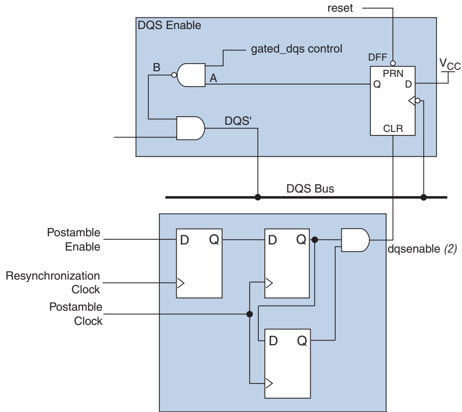
Figure 8–15. Stratix III DQS Postamble Circuitry Note (1)
