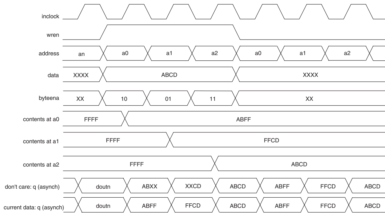
Figure 4–1. Stratix III Byte Enable Functional Waveform
