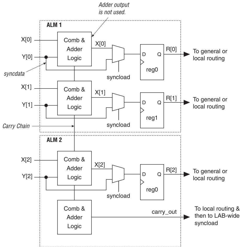
Figure 2–12. Conditional Operation Example
