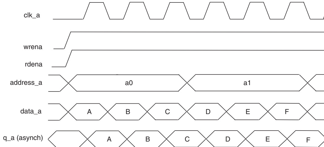
Figure 4–16. Same Port Read-During Write: New Data Mode
