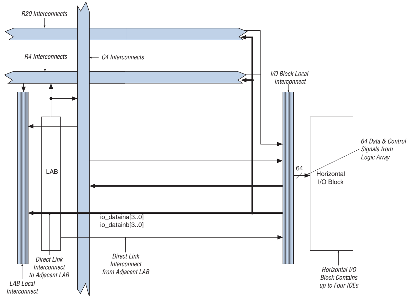
Figure 3–9. Row I/O Block Connection to Interconnect
