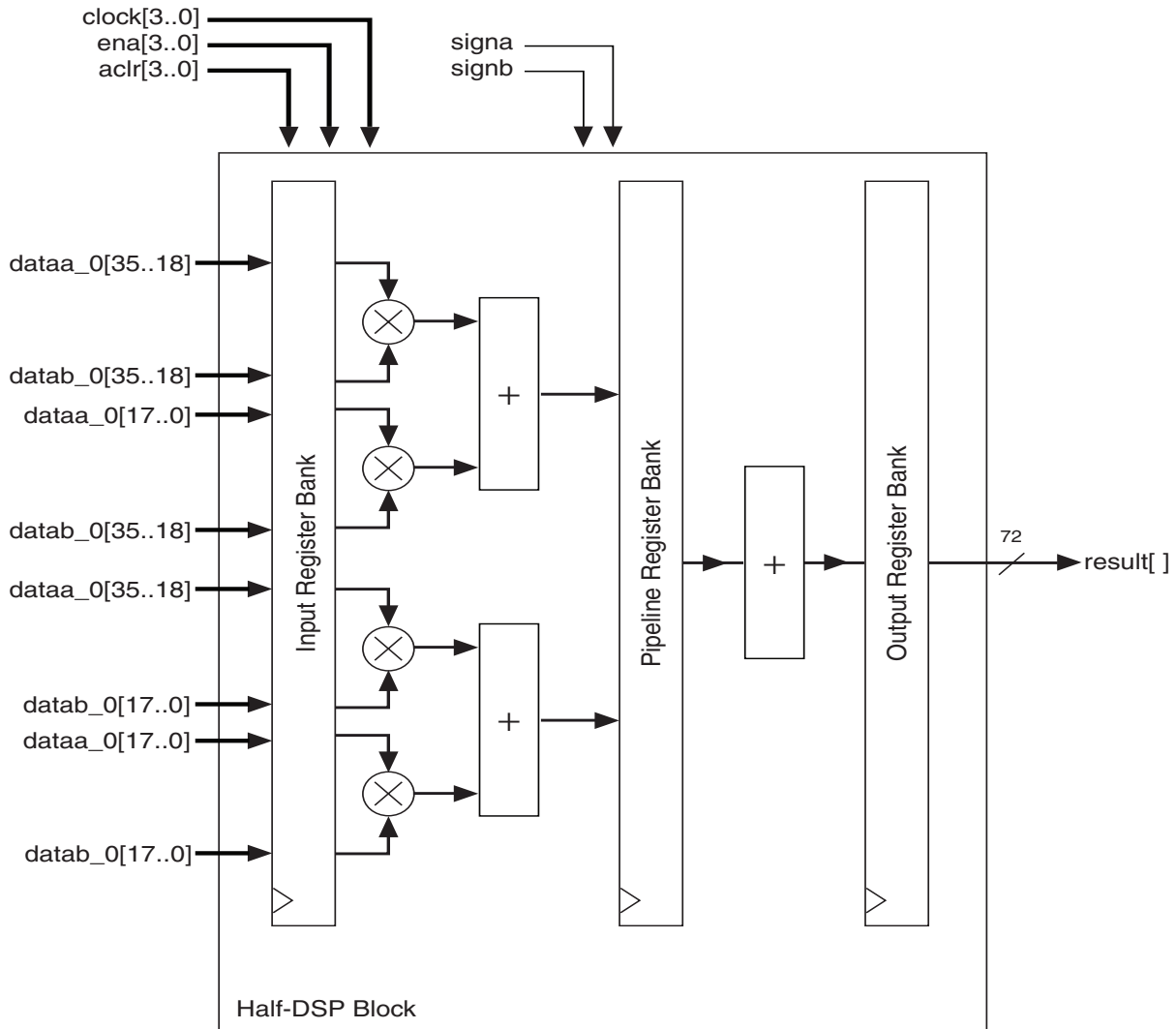
Figure 5–12. Double Mode Shown for Half-DSP Block
