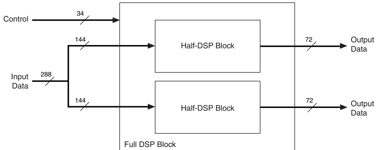
Figure 5-1. Overview of DSP Block Signals
