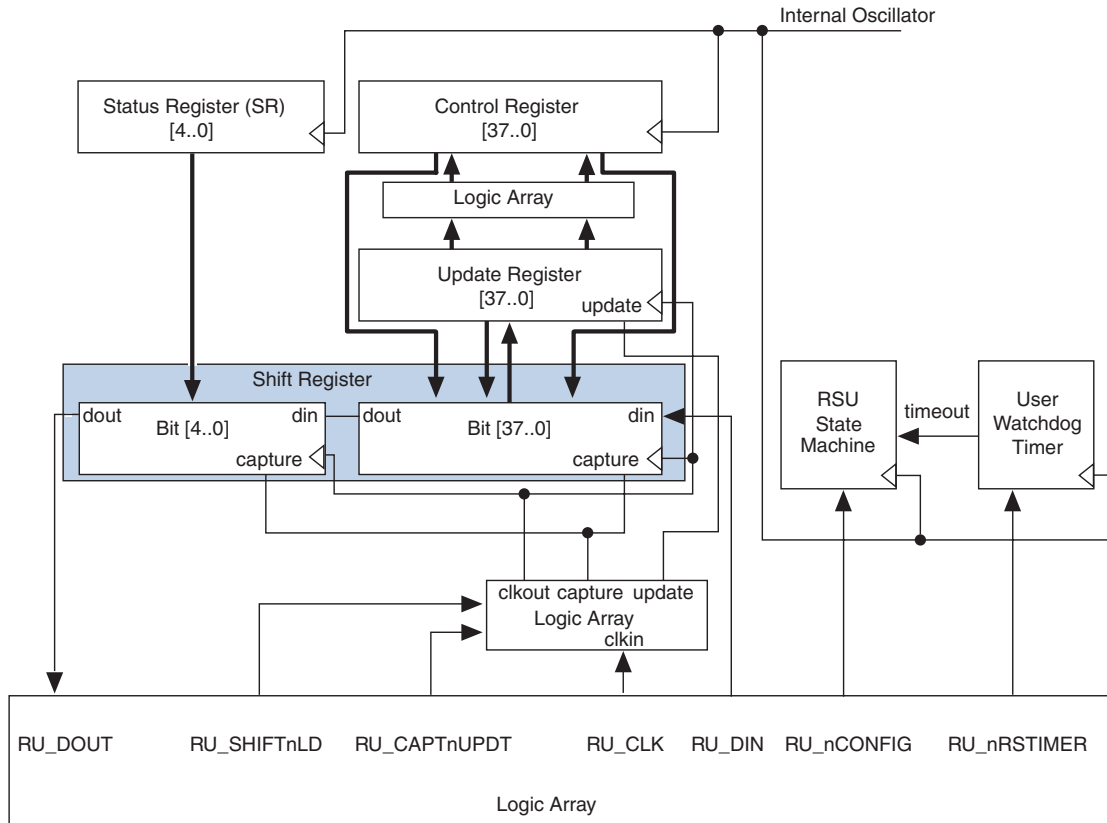
Figure 12–5. Remote System Upgrade Circuit Data Path Note (1)
