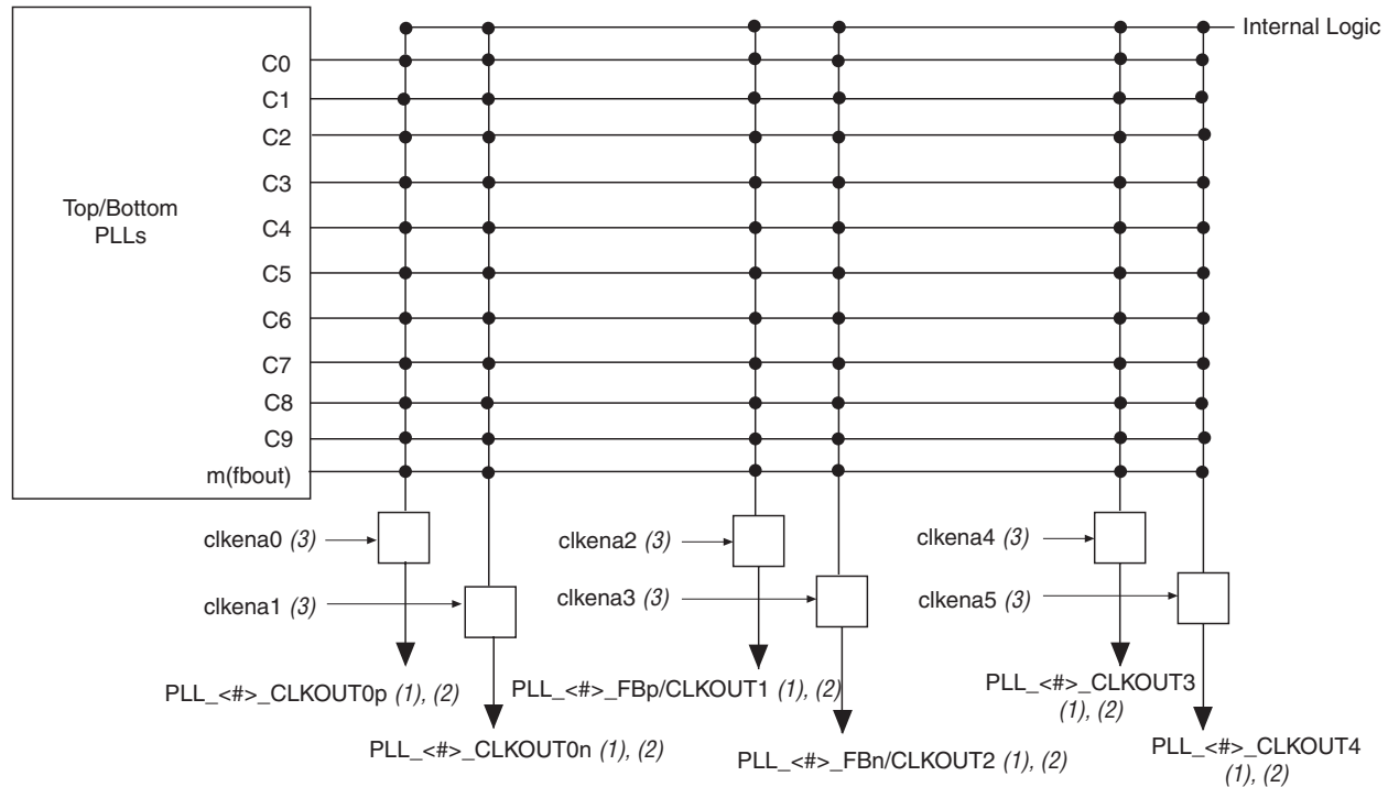
Figure 6–18. External Clock Outputs for Top/Bottom PLLs
