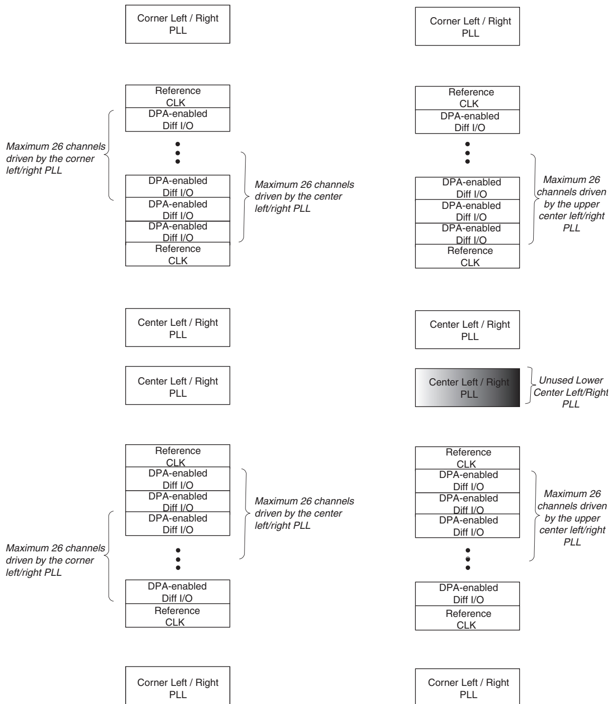
Figure 9–19. Left/Right PLL Driving Distance for DPA-Enabled Channels
