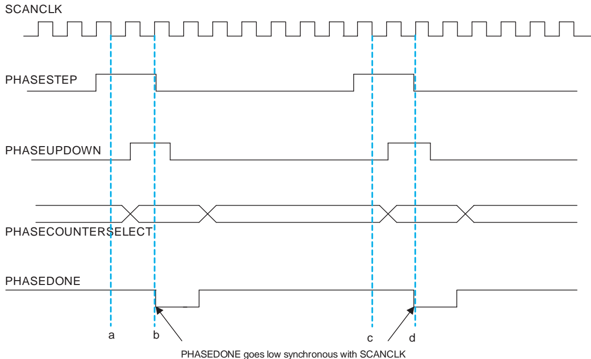
Figure 6–41. Dynamic Phase Shifting Waveform
