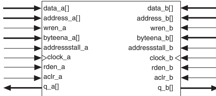
Figure 4–12. Stratix III True Dual-Port Memory Note (1)
