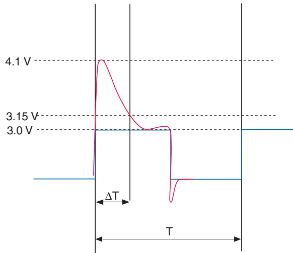
Figure 1–1. Overshoot Duration
