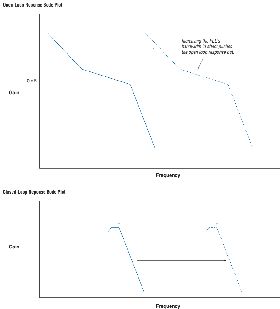
Figure 6–34. Open- and Closed-Loop Response Bode Plots
