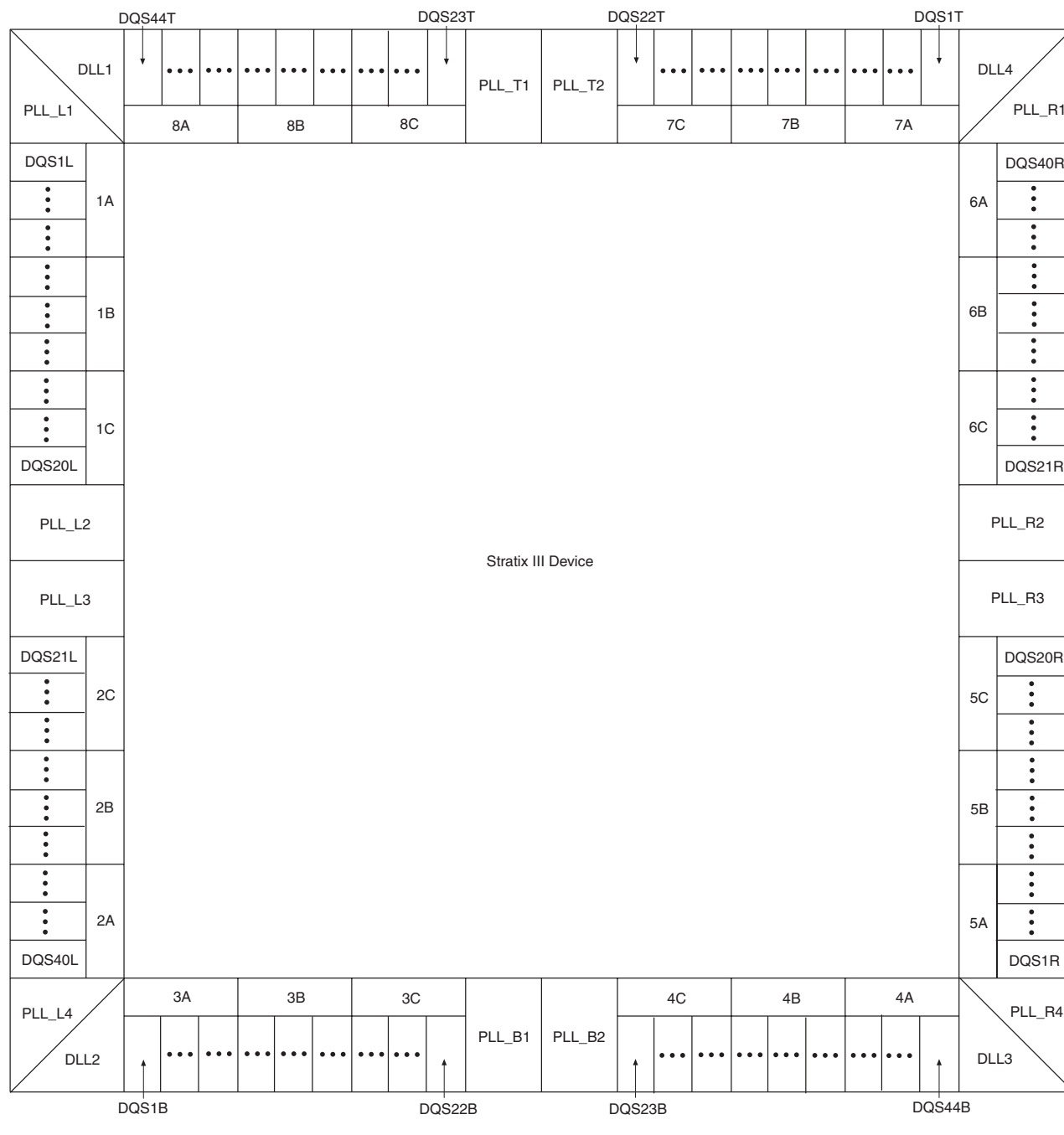
Figure 8–8. DQS Pins in Stratix III I/O Banks
