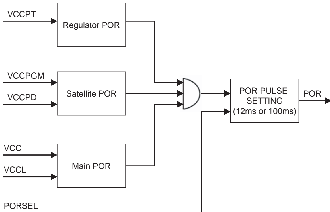
Figure 10-3. Simplified POR Block Diagram
