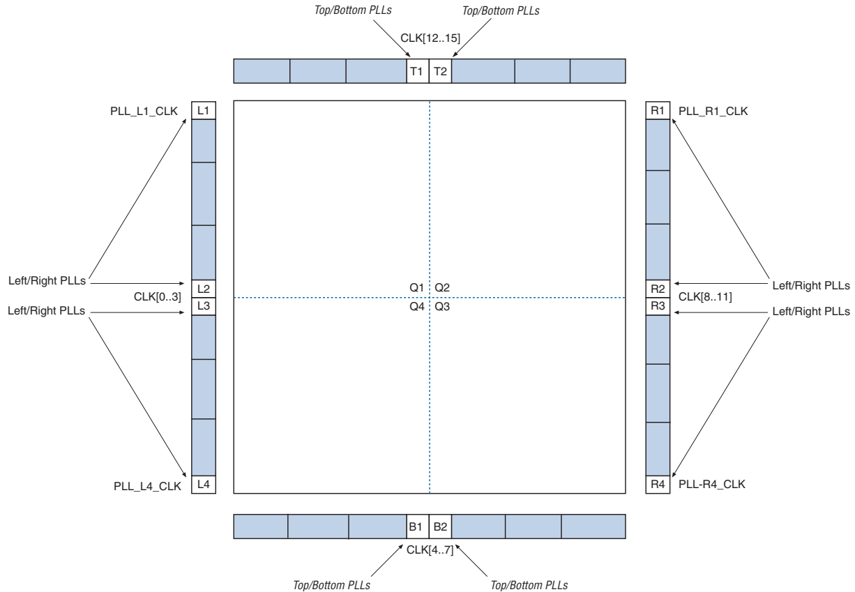
Figure 6–16. Stratix III PLL Locations
