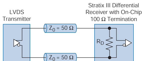
Figure 9–11. On-Chip Differential I/O Termination
