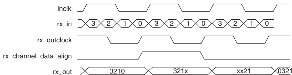
Figure 9–7. Data Realignment Timing
