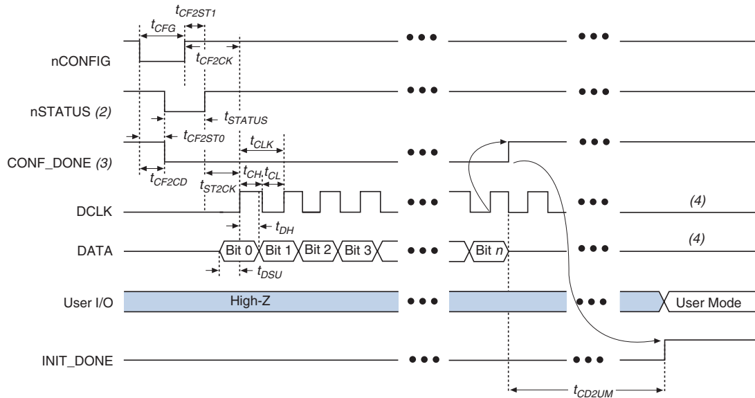
Figure 11–16. PS Configuration Timing Waveform (1)
