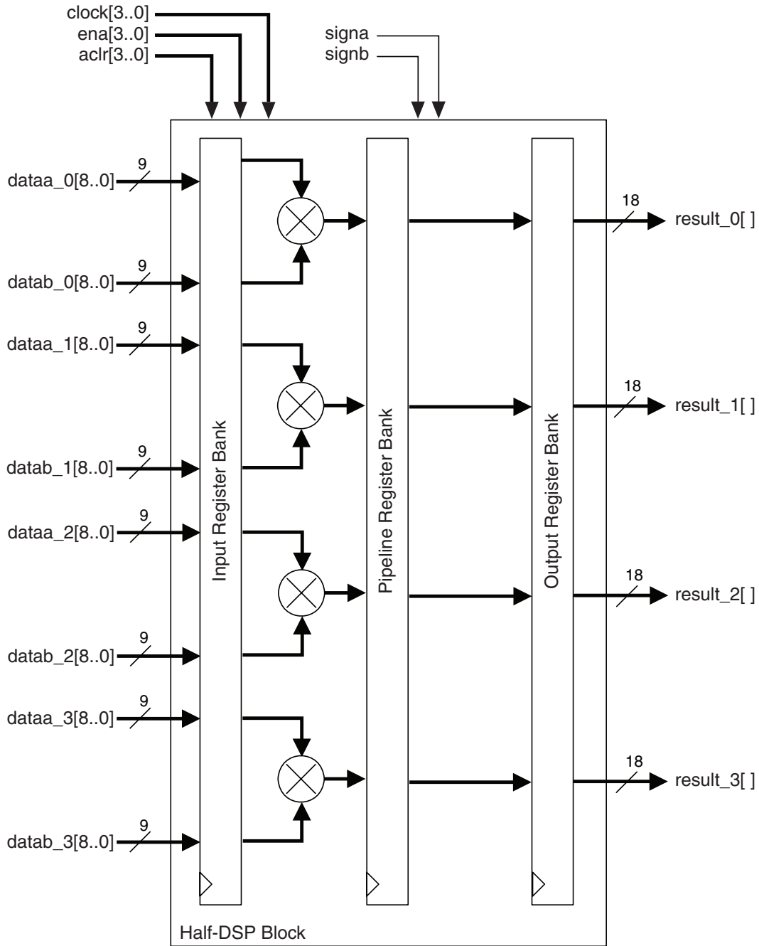
Figure 5–10. 9-Bit Independent Multiplier Mode Shown for Half-Block
