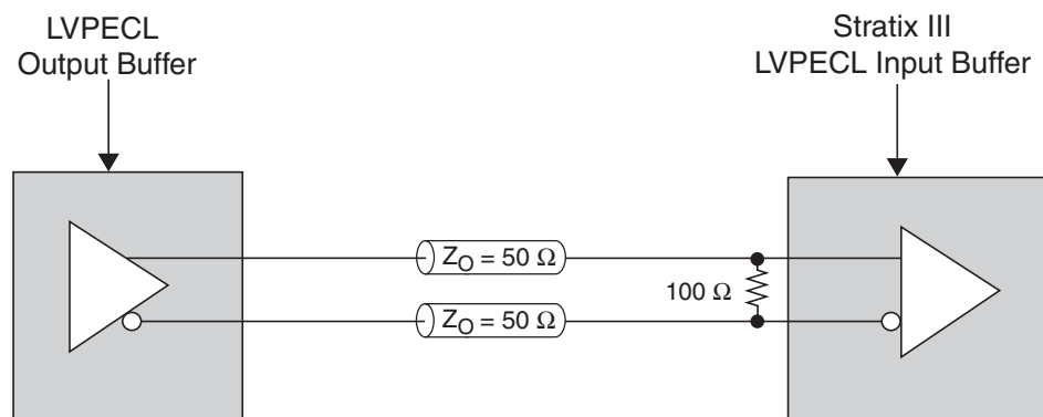
Figure 7–27. LVPECL DC Coupled Termination
