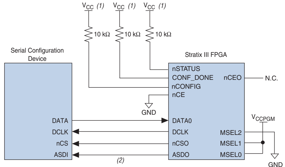
Figure 11–8. Single Device Fast AS Configuration
