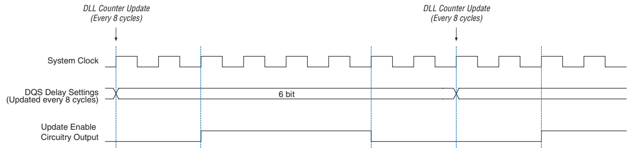
Figure 8–14. DQS Update Enable Waveform
