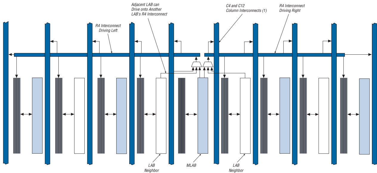
Figure 3–1. R4 Interconnect Connections Notes (1), (2)
