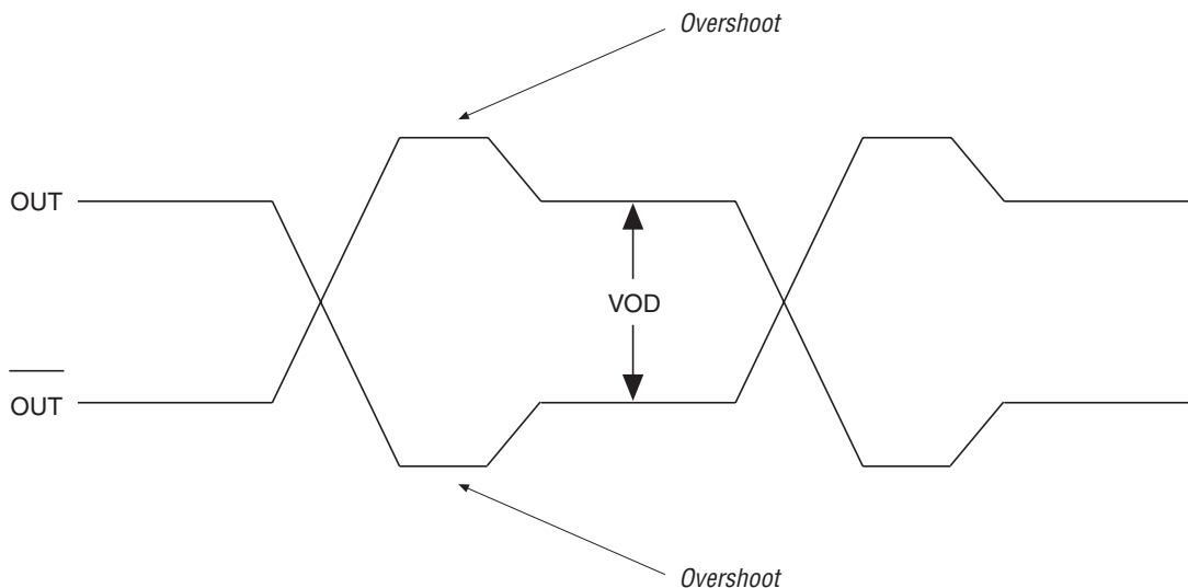
Figure 9–10. Programmable VOD
