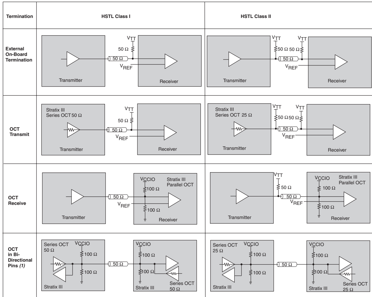
Figure 7–22. Stratix III HSTL I/O Standard Termination
