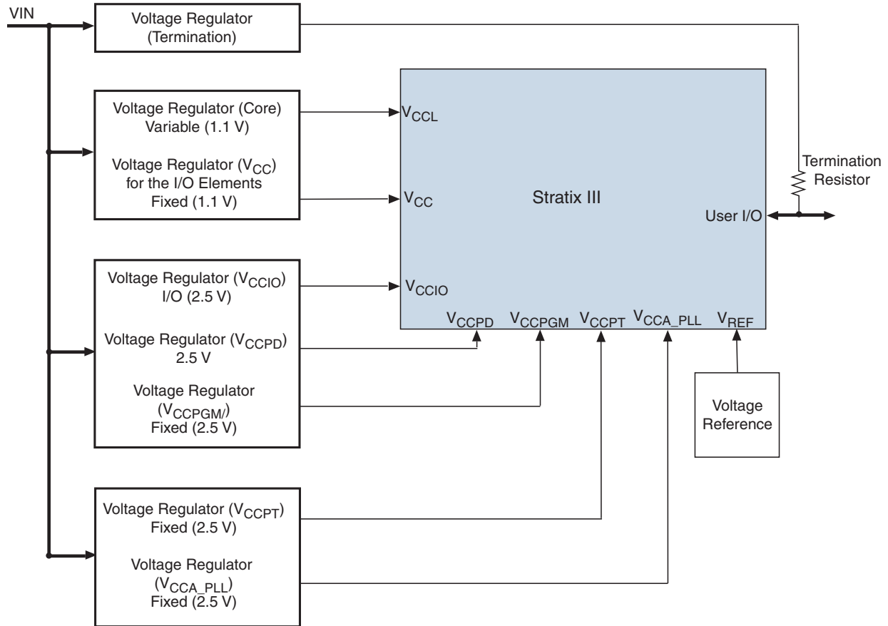
Figure 16–1. Stratix III Power Management Example
