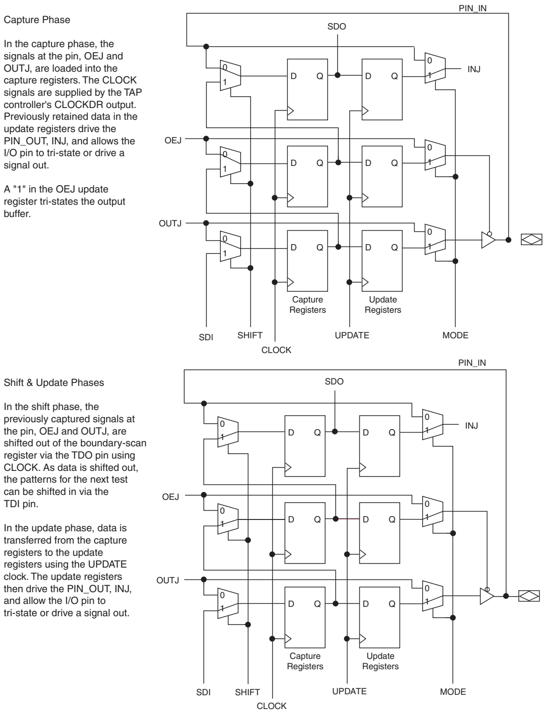
Figure 13–10. IEEE Std. 1149.1 BST EXTEST Mode
