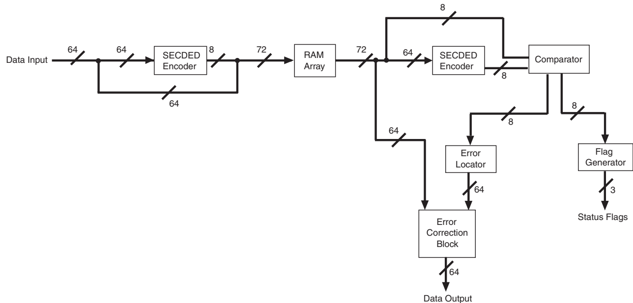
Figure 4–6. ECC Block Diagram of the M144K
