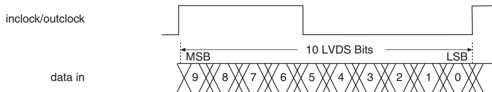
Figure 9–15. Bit Orientation in Quartus II Software
