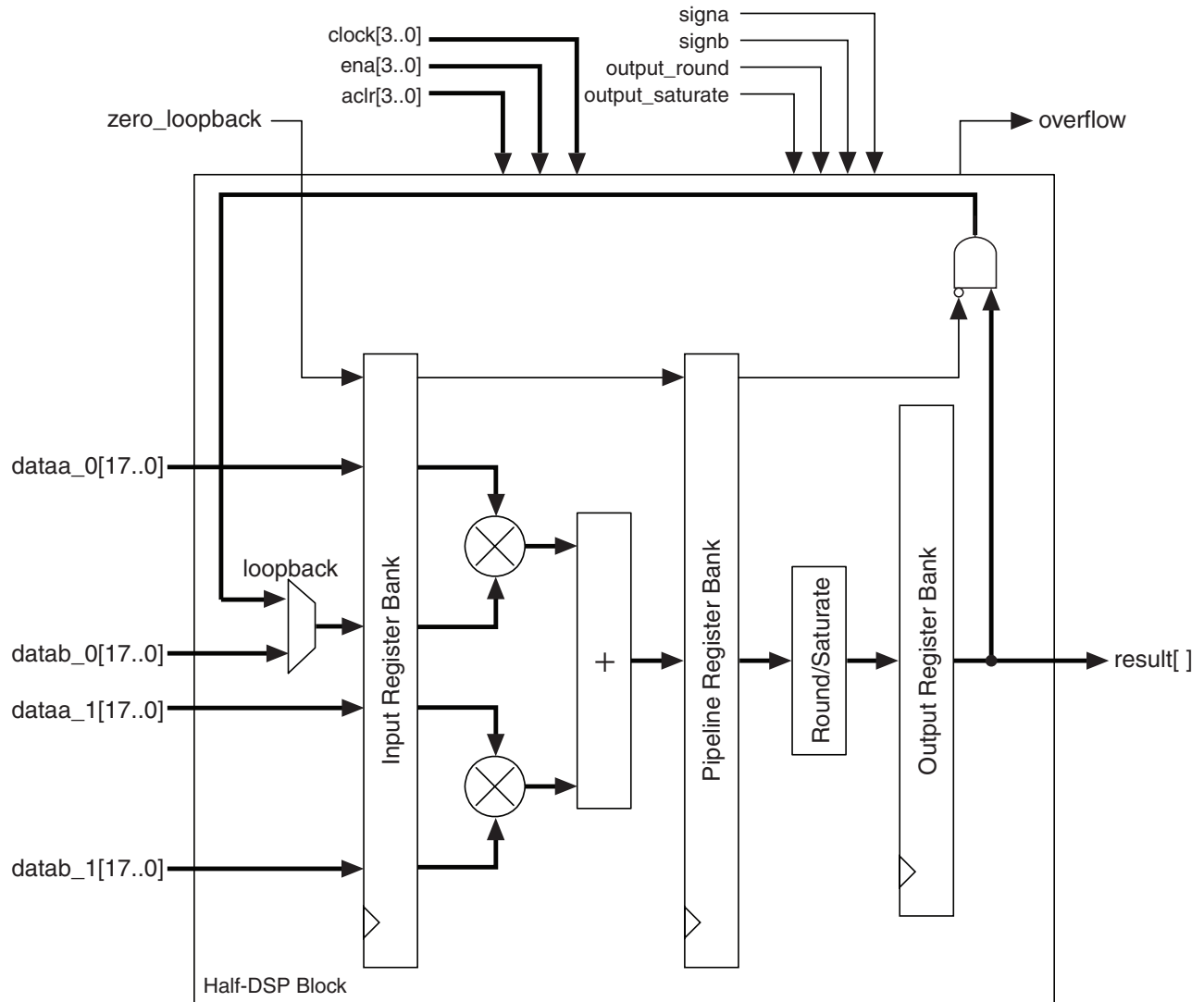
Figure 5–15. Loopback Mode for Half-DSP Block
