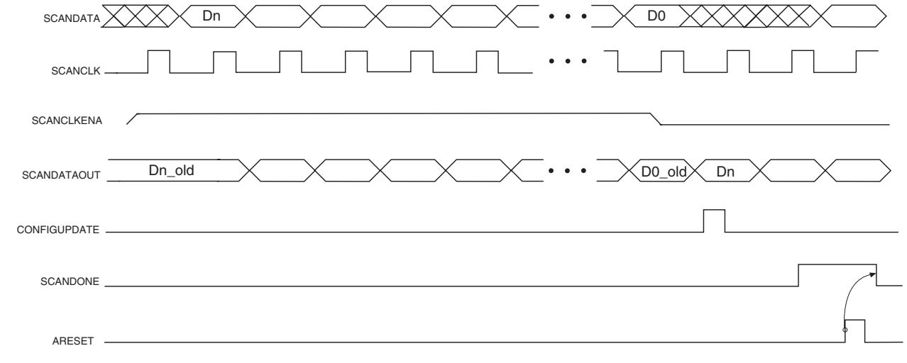
Figure 6–38. PLL Reconfiguration Waveform
