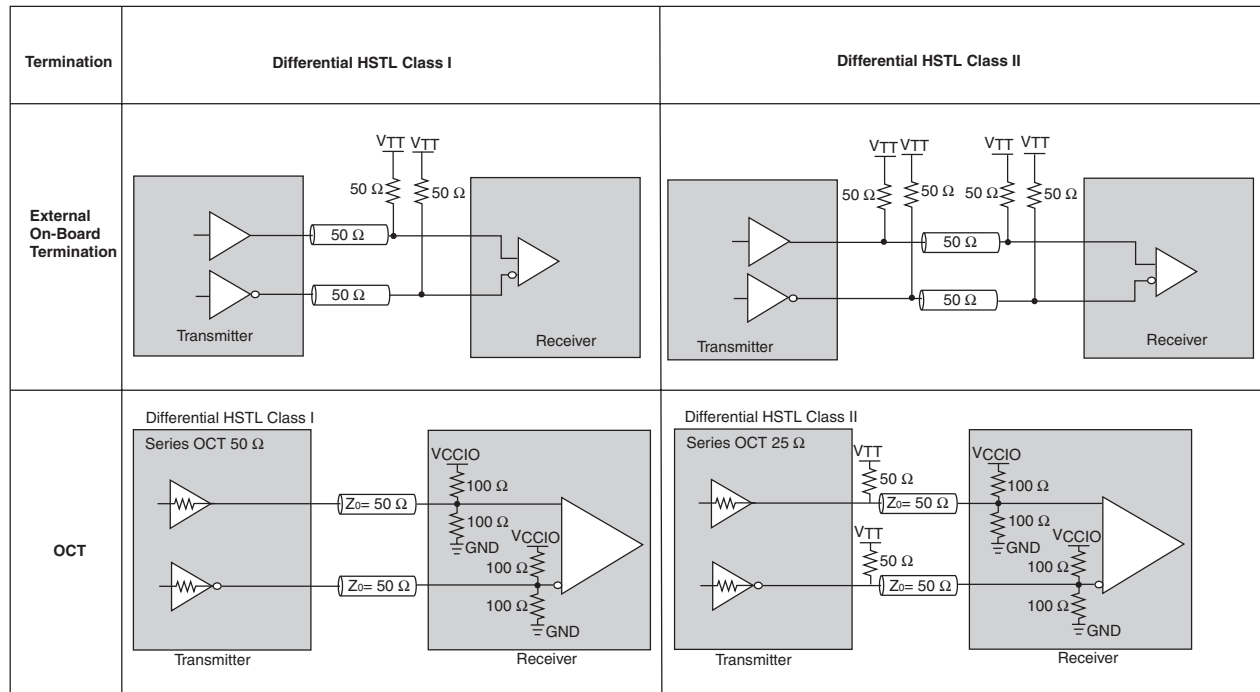
Figure 7–24. Stratix III Differential HSTL I/O Standard Termination
