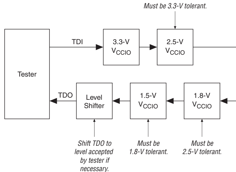
Figure 13–13. JTAG Chain of Mixed Voltages
