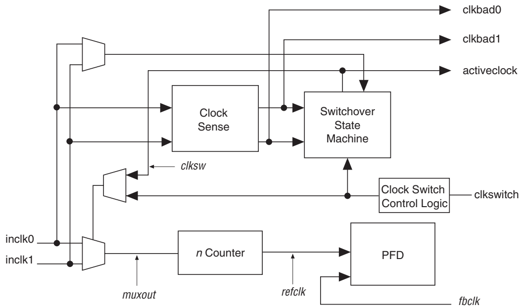
Figure 6–29. Automatic Clock Switchover Circuit Block Diagram
