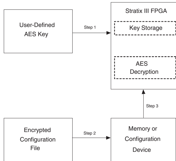
Figure 14–1. Design Security Note (1)
