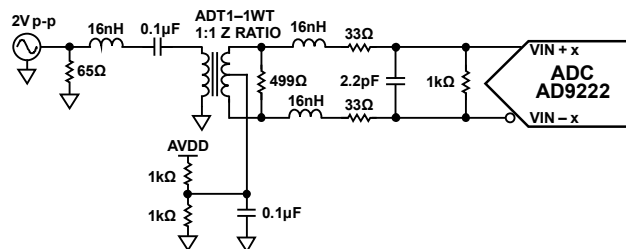
Figure 60. Differential Transformer-Coupled Configuration for IF Applications
