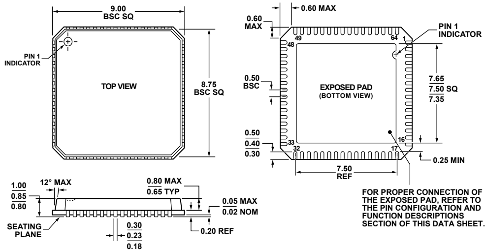
Figure 102. 64-Lead Lead Frame Chip Scale Package [LFCS_P_VQ] 9 mm × 9 mm Body, Very Thin Quad (CP-64-6) Dimensions shown in millimeters
