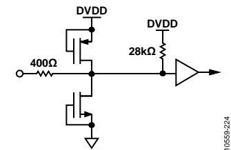
Figure 33. Equivalent \overline{CS} or \overline{RST} Input Circuit
