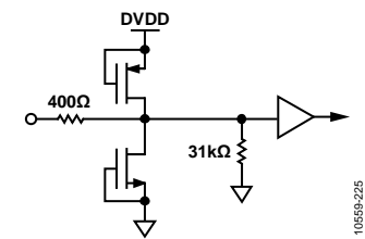
Figure 32. Equivalent SCLK or PDWN Input Circuit
