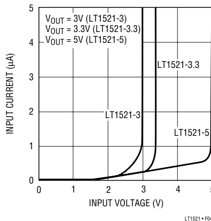
Figure 4. Input Current
