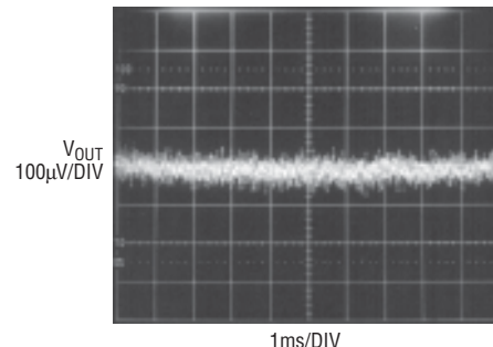
LT1761-5 10Hz to 100kHz Output Noise C_{BYYP} = 0.01\mu\text{F}
