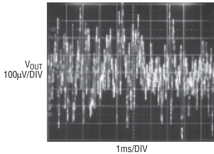
LT1761-5 10Hz to 100kHz Output Noise C_{BYYP} = 0
