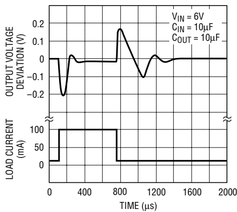
LT1761-5 Transient Response C_{BYYP} = 0
