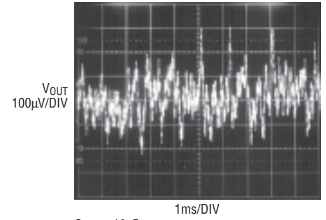
LT1761-5 10Hz to 100kHz Output Noise C_{BYYP} = 100\text{pF}
