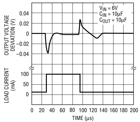
LT1761-5 Transient Response C_{BYYP} = 0.01\mu\text{F}
