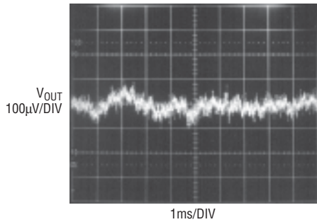
LT1761-5 10Hz to 100kHz Output Noise C_{BYYP} = 1000\text{pF}
