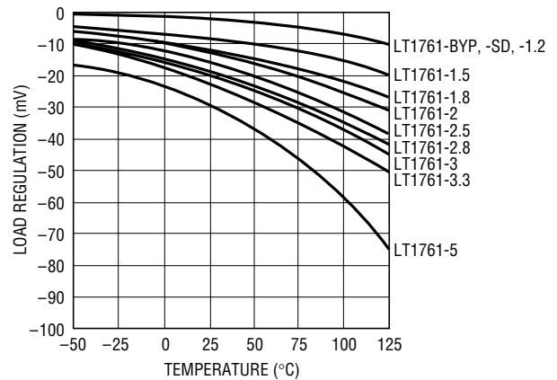
Load Regulation \Delta I_L = 1\text{mA} to 100\text{mA}
