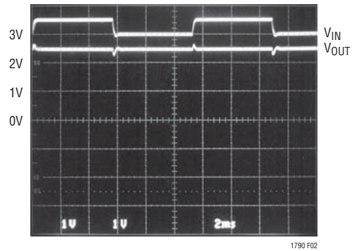
Figure 2. Output Response to 0.5V Ripple on V_{IN}
