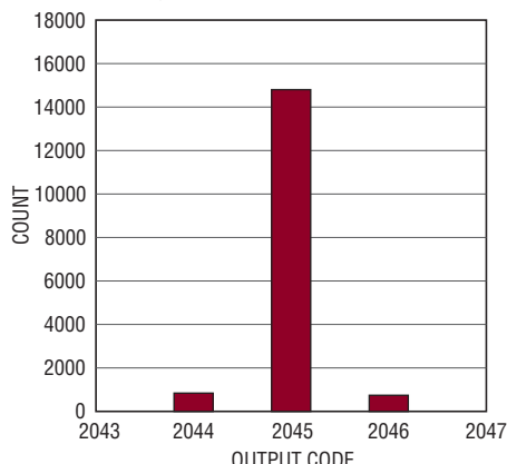
LTC2142-12: Shorted Input Histogram
