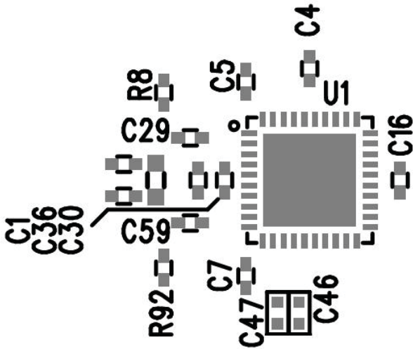
Silkscreen Top
