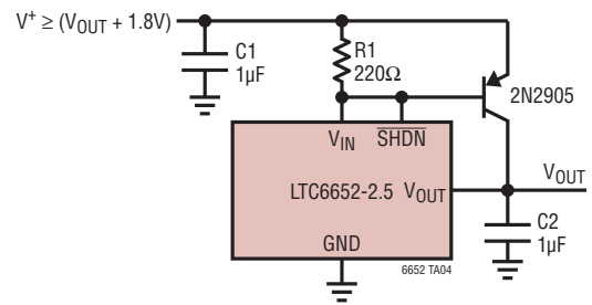
Boosted Output Current
