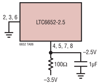
Negative Rail Circuit
