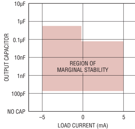
Stability with Output Capacitance (LTC6652-2.5, LTC6652-3, LTC6652-3.3, LTC6652-4.906, LTC6652-5)
