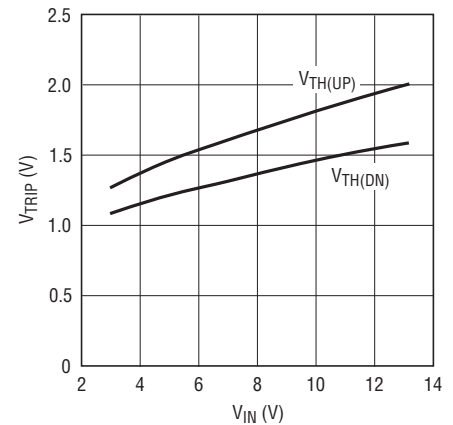
SHDN Input Voltage Thresholds vs V_{IN}
