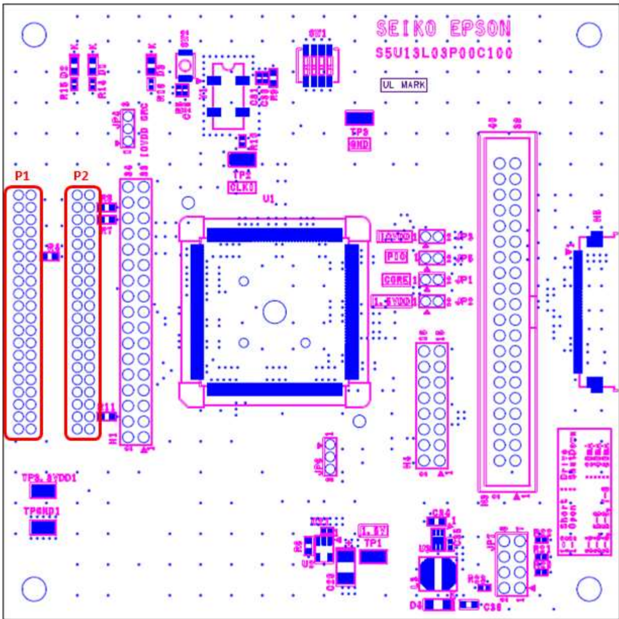
Figure 4-2: USB Adapter Connector Locations (P1 and P2)
