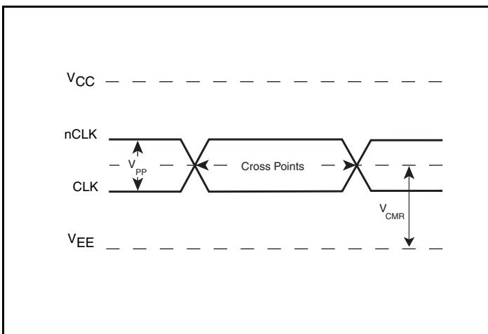
Differential Input Levels
