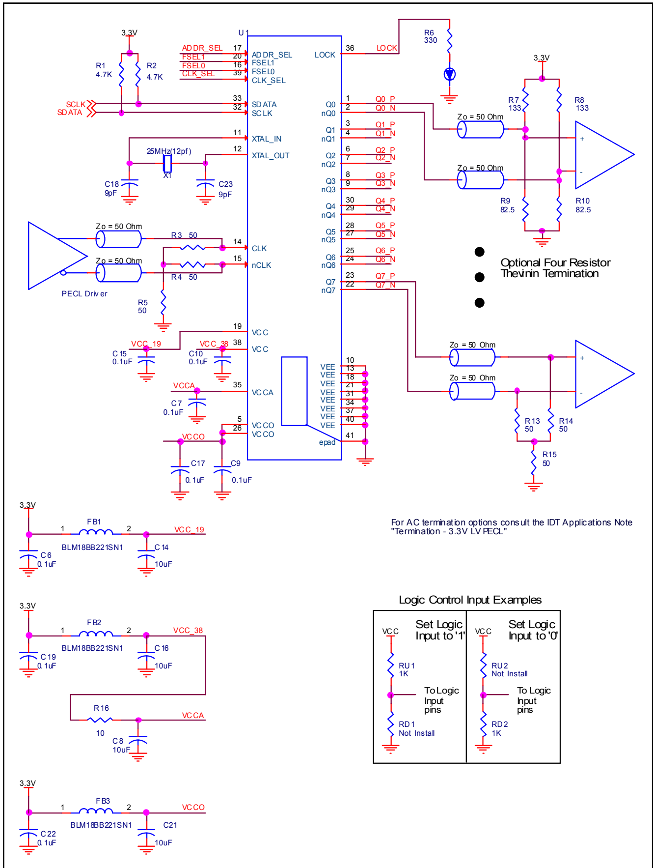
Figure 9. IDT8T49N008I Application Schematic
