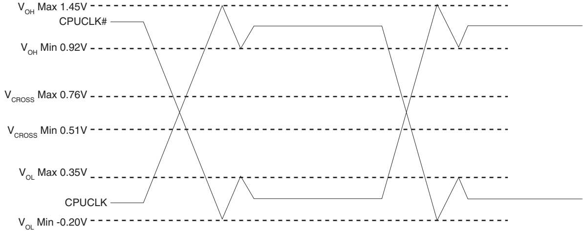
Figure 5 - 1.0V Single Ended VCross, VOH and VOL Measurement Points
