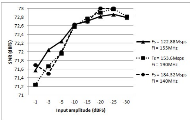
Fig 19. SNR as a function of input amplitude: V_{L(dif)} = 2 V
