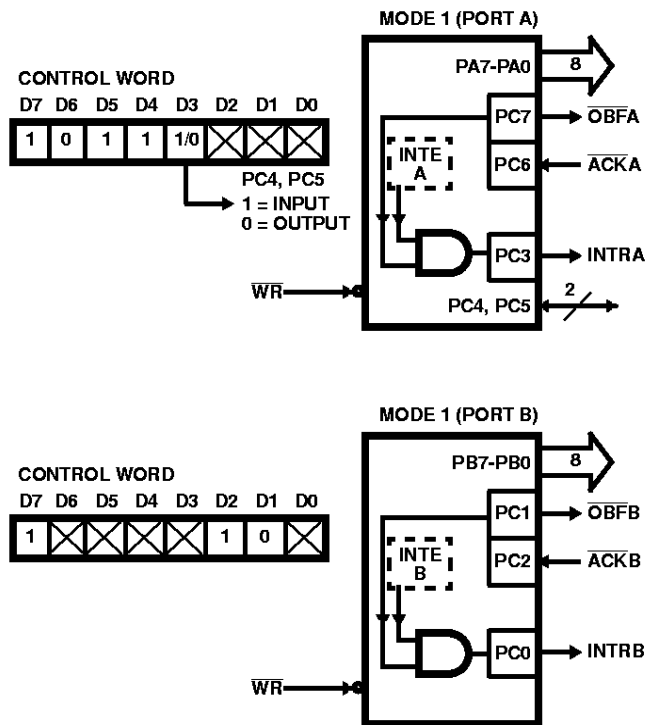
FIGURE 8. MODE 1 OUTPUT
