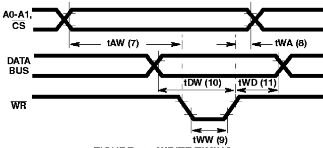
FIGURE 30. WRITE TIMING
