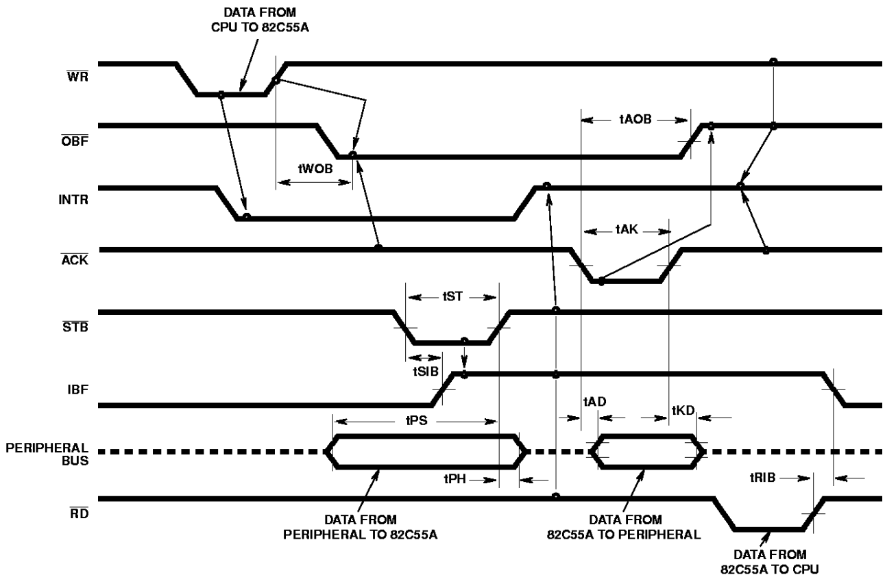
FIGURE 13. MODE 2 (BI-DIRECTIONAL)
