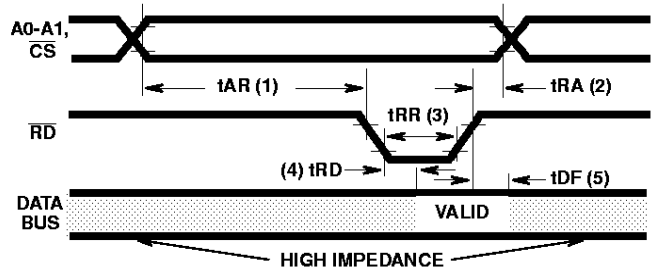
FIGURE 31. READ TIMING
