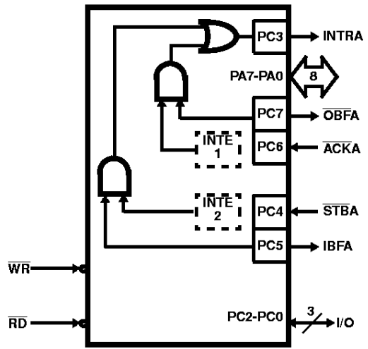
FIGURE 12. MODE 2
