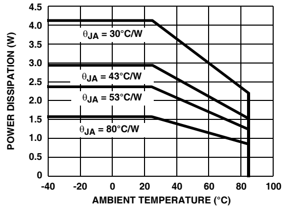
FIGURE 40. POWER DISSIPATION vs AMBIENT TEMPERATURE for VARIOUS MOUNTED \theta_{JA} s (See Thermal Resistance Curve on page 15)
