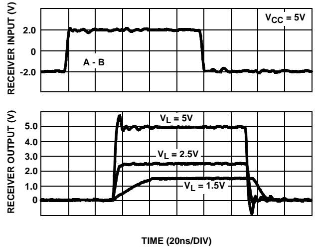
FIGURE 15. RECEIVER WAVEFORMS
