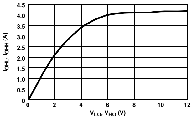
FIGURE 14. PEAK PULL-DOWN CURRENT vs OUTPUT VOLTAGE
