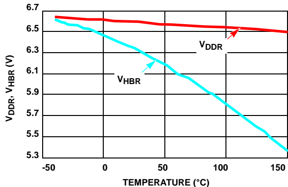
FIGURE 9. UNDERVOLTAGE LOCKOUT THRESHOLD vs TEMPERATURE
