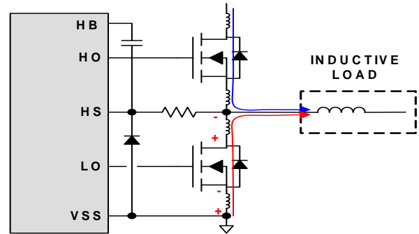
FIGURE 20. PARASITIC INDUCTANCE CAUSES TRANSIENTS ON HS NODE
