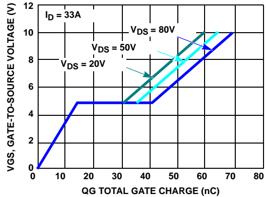
FIGURE 18. TYPICAL GATE CHARGE OF A POWER FET
