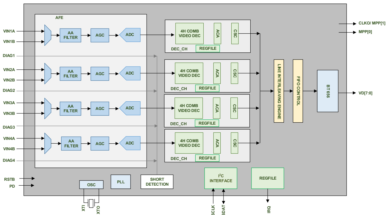
FIGURE 2. ISL79986 BLOCK DIAGRAM
