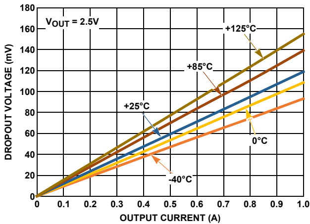
FIGURE 4. DROPOUT vs OUTPUT CURRENT
