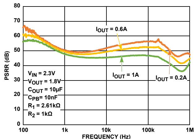
FIGURE 2. PSRR
