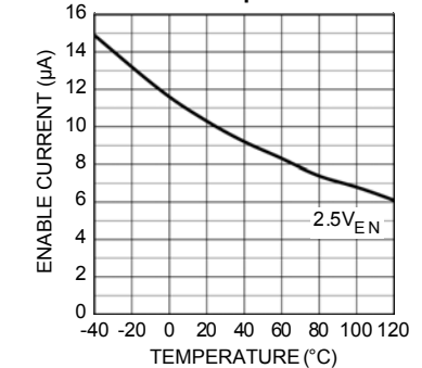
Enable Current vs. Temperature
