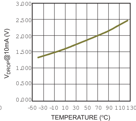
Voltage Drop at Bootstrap Switch vs. Temperature
