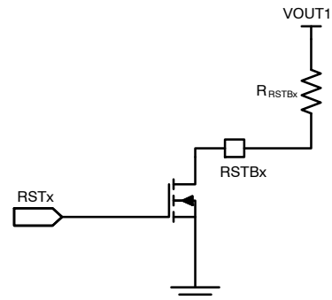
Figure 27. Reset Delay Time
