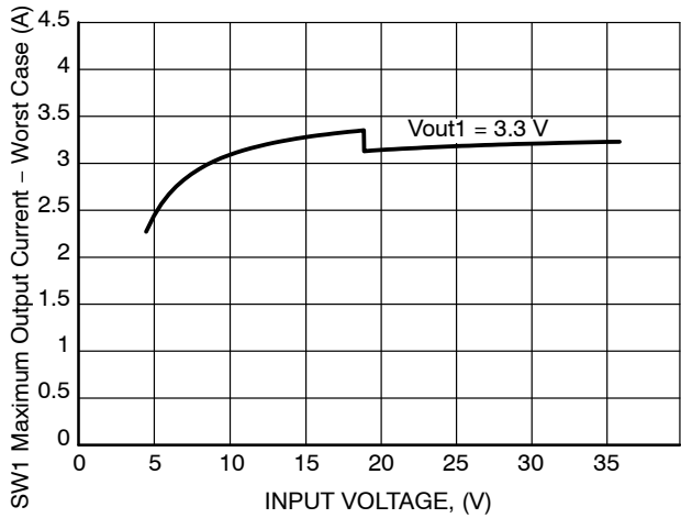
Figure 30. Switcher 1 Load Current Capability with a 4.7 \mu\text{H} Inductor
