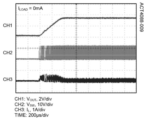
Start-up Waveforms
