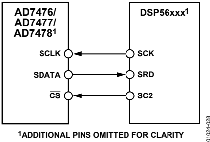
Figure 28. Interfacing to the DSP56xxx
