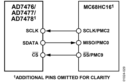
Figure 29. Interfacing to the MC68HC16
