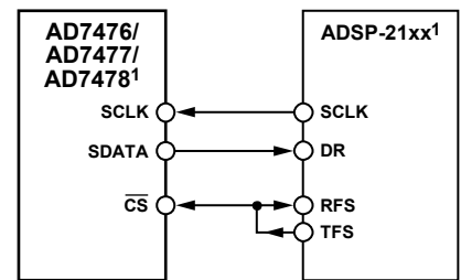
1 ADDITIONAL PINS OMITTED FOR CLARITY Figure 27. Interfacing to the ADSP-21xx
