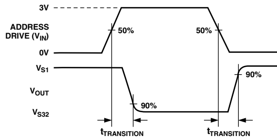
Test Circuit 5. Switching Time of Multiplexer, t_{TRANSITION}
