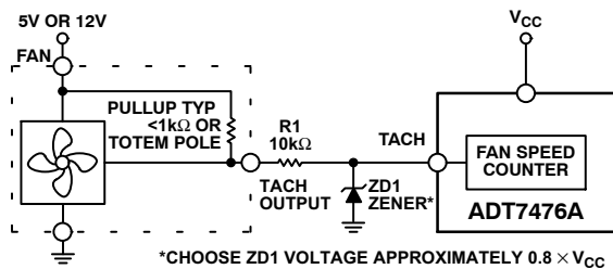
Figure 43. Fan with Strong TACH Pullup to >V CC or Totem-Pole Output, Clamped with Zener Diode and Resistor
