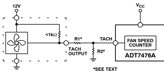
Figure 44. Fan with Strong TACH Pullup to >V CC or Totem-Pole Output, Attenuated with R1/R2
