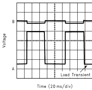
V_{O5} Load Transient Response
