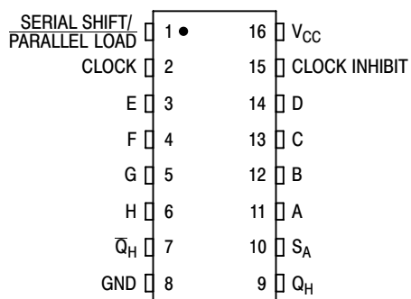
Figure 1. Pin Assignment
