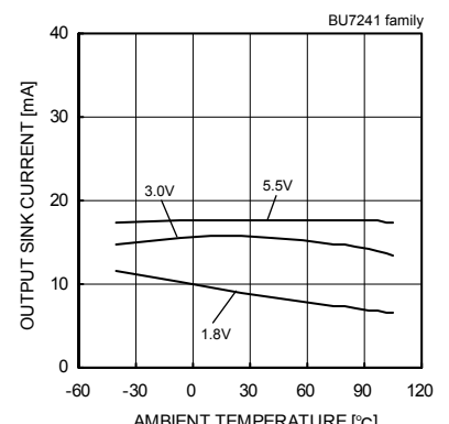
Fig. 58 Output Sink Current - Ambient Temperature (VOUT=VSS+0.4[V])
