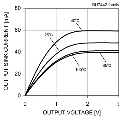
Fig. 172 Output Sink Current - Output Voltage (VDD=3[V])
