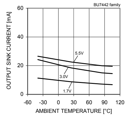
Fig. 173 Output Sink Current - Ambient Temperature (VOUT=VSS+0.4[V])
