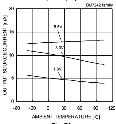
Fig. 79 Output Source Current - Ambient Temperature (VOUT=VDD-0.4[V])
