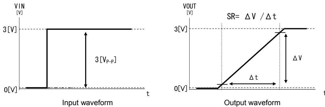
Fig. 187. Slew rate input output wave
