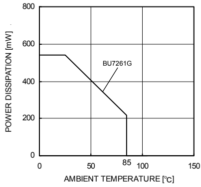
Fig. 1 Derating curve
