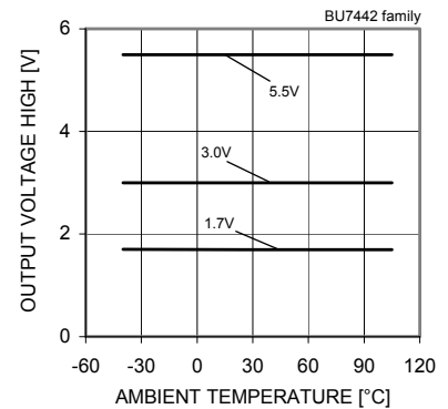
Fig. 167 Output Voltage High - Ambient Temperature (RL=10[kΩ])
