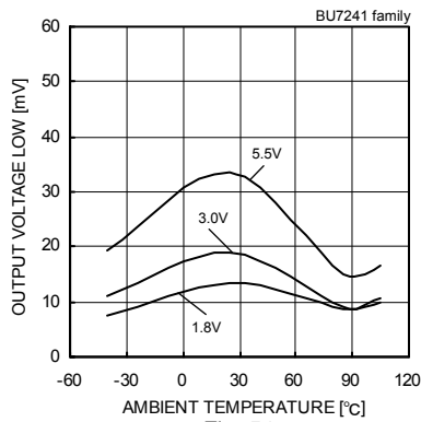
Fig. 54 Output Voltage Low - Ambient Temperature (RL=10[kΩ])
