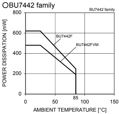
Fig. 162 Derating curve
