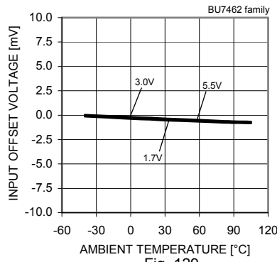
Fig. 129 Input Offset Voltage – Ambient Temperature (Vicm=VDD-1.2[V], VOUT= VDD/2)
