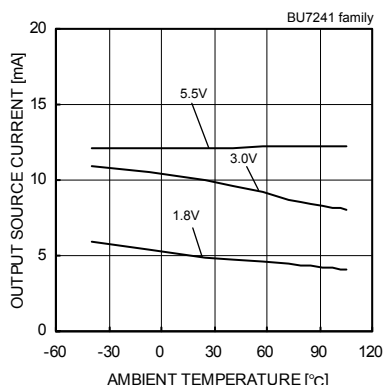
Fig. 56 Output Source Current - Ambient Temperature (VOUT=VDD-0.4[V])
