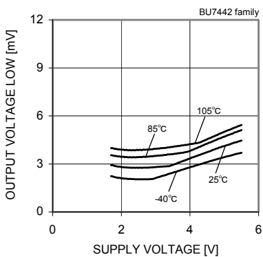
Fig. 168 Output Voltage Low - Supply Voltage (RL=10[kΩ])
