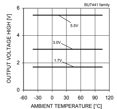
Fig. 144 Output Voltage High - Ambient Temperature (RL=10[kΩ])
