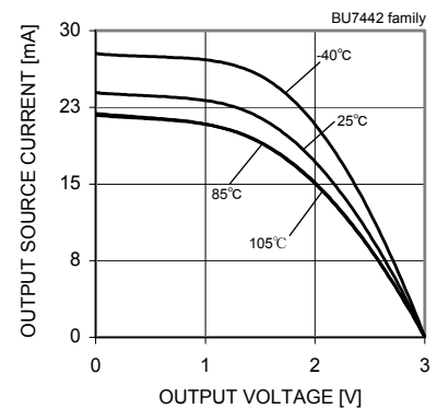
Fig. 170 Output Source Current - Output Voltage (VDD=3.0[V])
