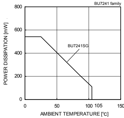
Fig. 48 Derating curve
