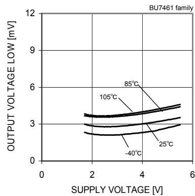
Fig. 99 Output Voltage Low - Supply Voltage ( R_L=10[k\Omega] )
