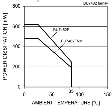
Fig. 116 Derating curve
