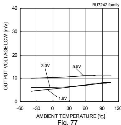
Fig. 77 Output Voltage Low - Ambient Temperature (RL=10[kΩ])
