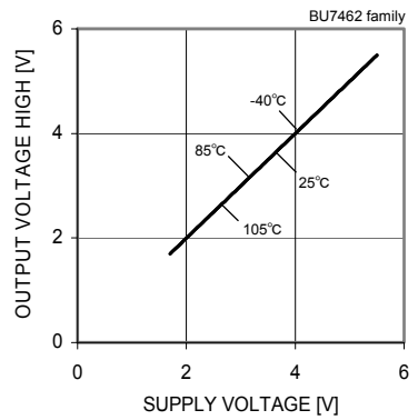
Fig. 120 Output Voltage High - Supply Voltage (RL=10[kΩ])
