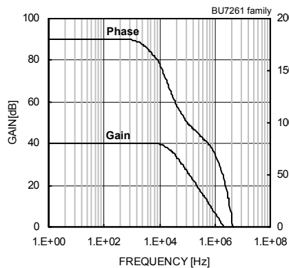
Fig. 23 Gain - Frequency
