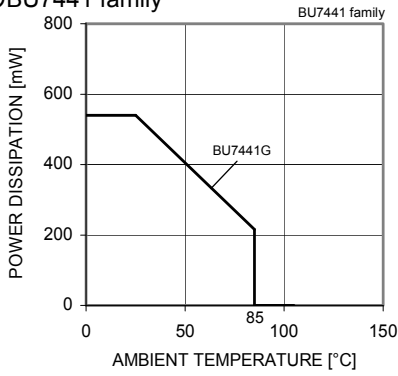
Fig. 139 Derating curve
