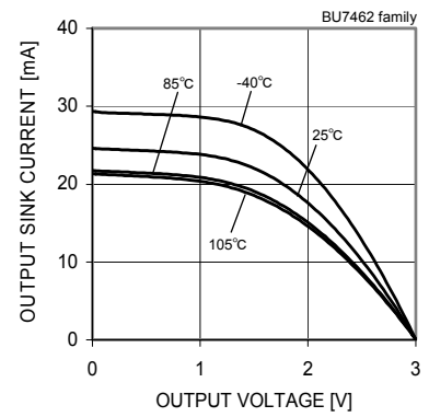
Fig. 124 Output Source Current - Output Voltage (VDD=3.0[V])
