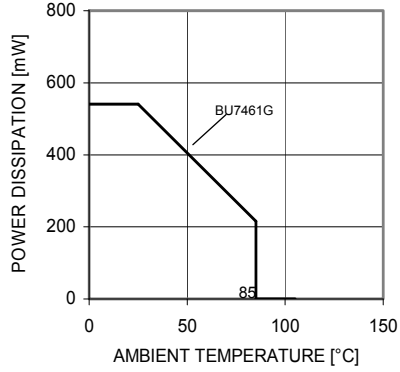
Fig. 93 Derating curve
