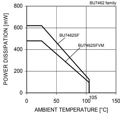
Fig. 117 Derating curve
