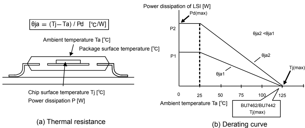
Fig. 190 Thermal resistance and derating
