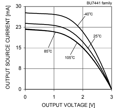
Fig. 147 Output Source Current - Output Voltage (VDD=3.0[V])
