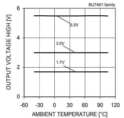
Fig. 98 Output Voltage High - Ambient Temperature
