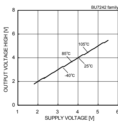
Fig. 74 Output Voltage High - Supply Voltage (RL=10[kΩ])
