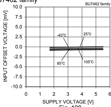
Fig. 128 Input Offset Voltage – Supply Voltage (Vicm=VDD-1.2[V], VOUT= VDD/2)
