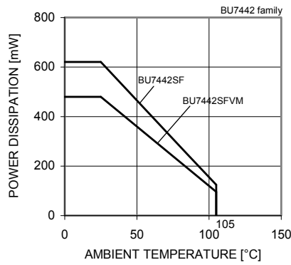
Fig. 163 Derating curve
