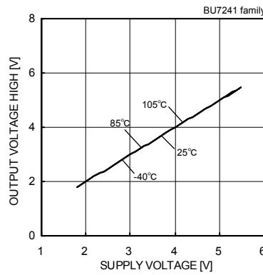
Fig. 51 Output Voltage High - Supply Voltage (RL=10[kΩ])
