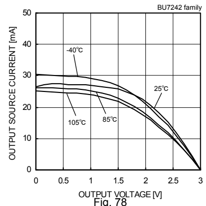
Fig. 78 Output Source Current - Output Voltage (VDD=3.0[V])
