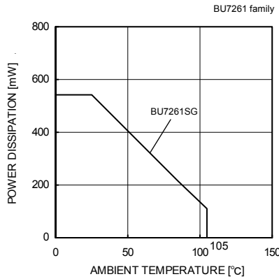
Fig. 2 Derating curve
