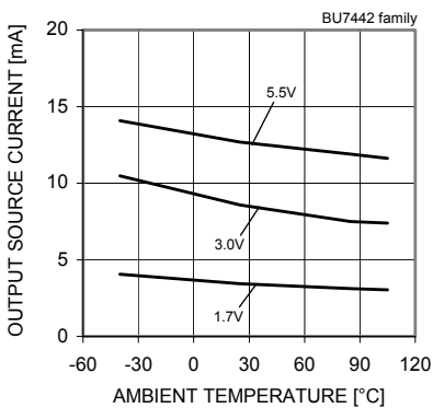
Fig. 171 Output Source Current - Ambient Temperature (VOUT=VDD-0.4[V])
