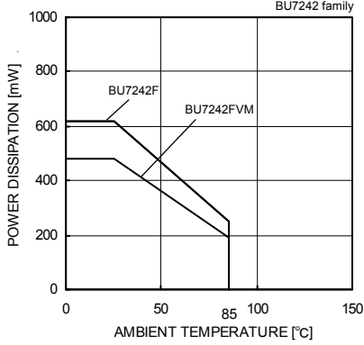
Fig. 70 Derating curve
