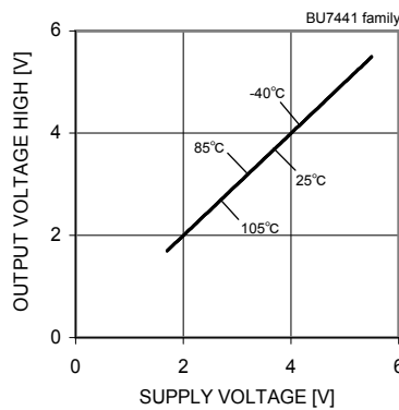
Fig. 143 Output Voltage High - Supply Voltage (RL=10[kΩ])
