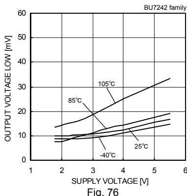
Fig. 76 Output Voltage Low - Supply Voltage (RL=10[kΩ])
