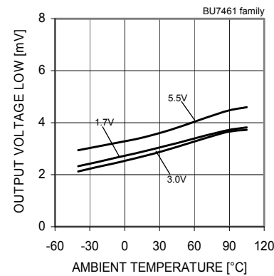
Fig. 100 Output Voltage Low - Ambient Temperature ( R_L=10[k\Omega] )
