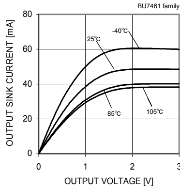
Fig. 103 Output Sink Current - Output Voltage ( V_{DD}=3[V] )
