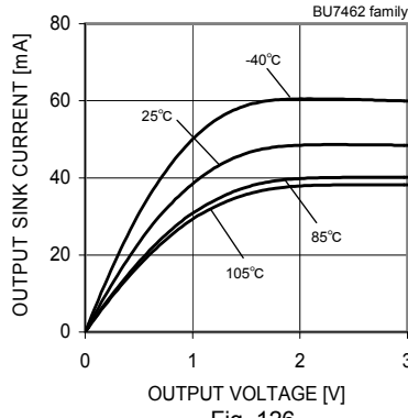
Fig. 126 Output Sink Current - Output Voltage (VDD=3[V])
