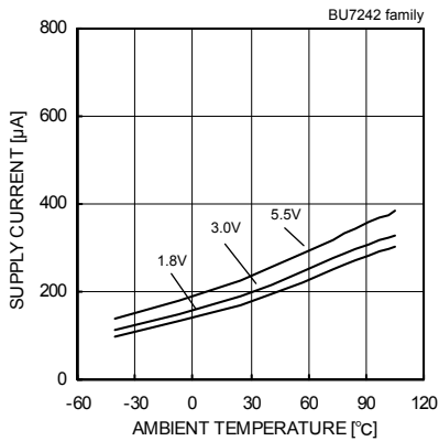
Fig. 73 Supply Current - Ambient Temperature
