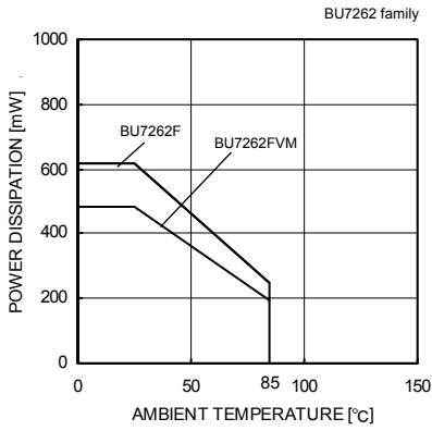
Fig. 24 Derating curve
