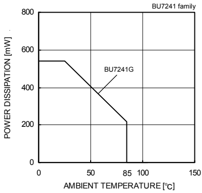
Fig. 47 Derating curve
