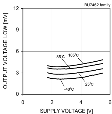
Fig. 122 Output Voltage Low - Supply Voltage (RL=10[kΩ])
