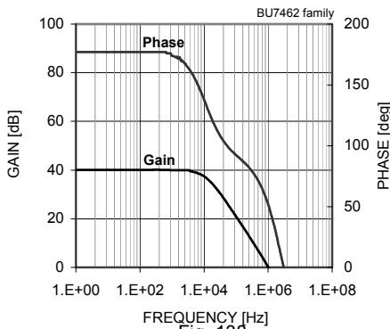
Fig. 138 Gain - Frequency
