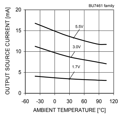
Fig. 102 Output Source Current - Ambient Temperature ( V_{OUT}=V_{DD}-0.4[V] )
