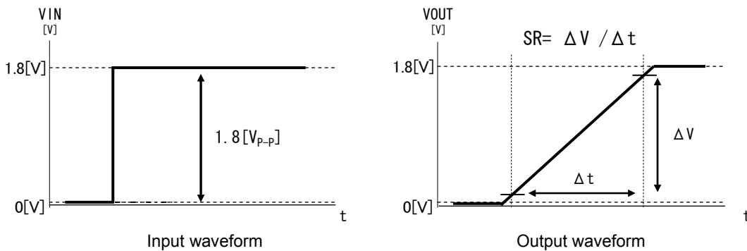
Fig. 188. Slew rate input output wave
