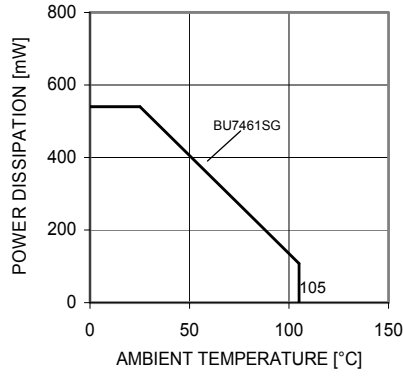
Fig. 94 Derating curve
