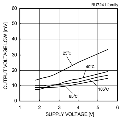
Fig. 53 Output Voltage Low - Supply Voltage (RL=10[kΩ])
