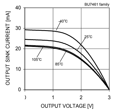
Fig. 101 Output Source Current - Output Voltage ( V_{DD}=3.0[V] )
