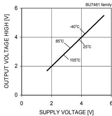
Fig. 97 Output Voltage High - Supply Voltage
