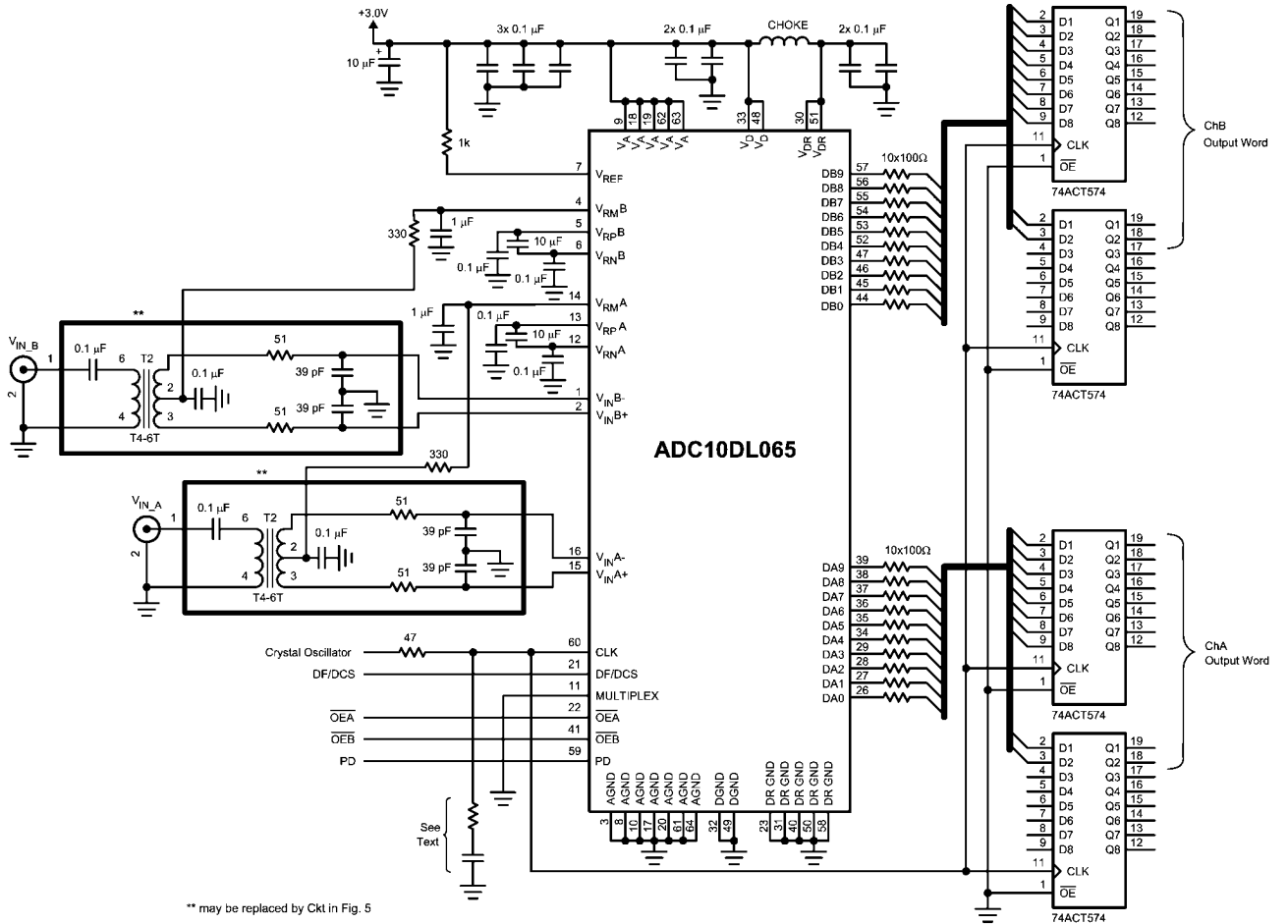
FIGURE 4. Application Circuit Using Transformer Drive Circuit, Parallel Mode
