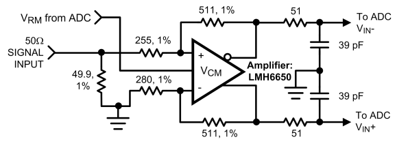
FIGURE 6. Optional Amplifier Differential Drive Circuit
