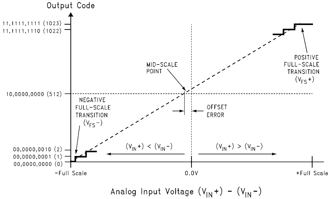
FIGURE 1. Transfer Characteristic
