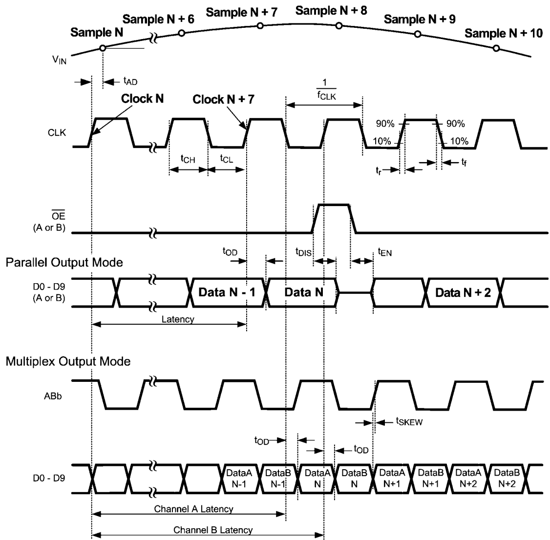
Output Timing
