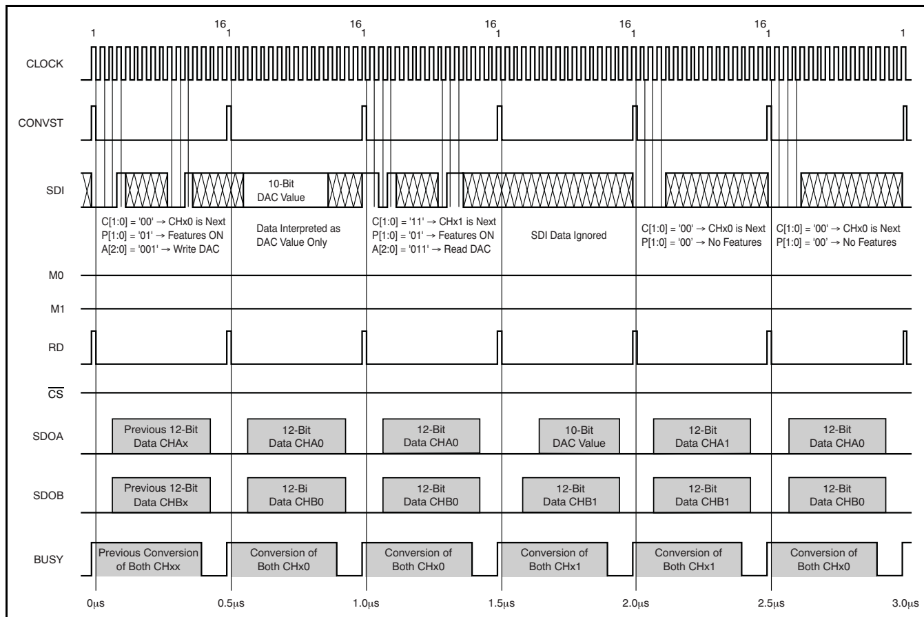
Figure 41. DAC Write and Read Access Timing Diagram
