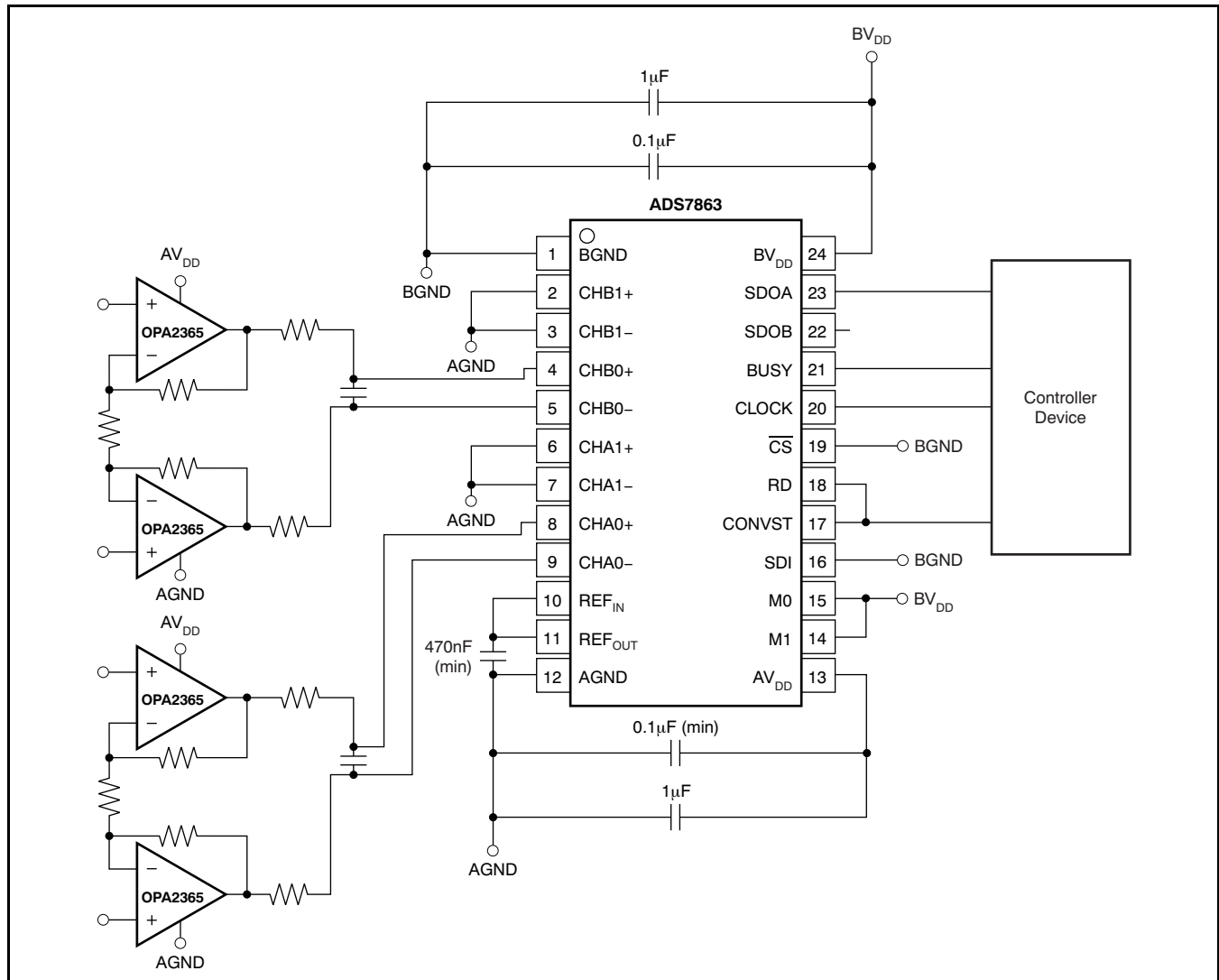
Figure 42. Minimum ADS7863 Configuration
