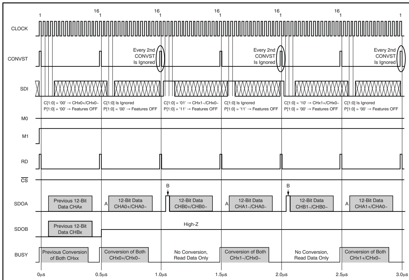
Figure 40. Pseudo-Differential Mode II (M0 = 0; M1 = 1)
