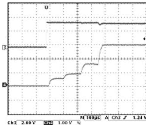
Start up into PWM Mode V_{OUT} = 3.0\text{ V}, 1.5A\text{ load}
