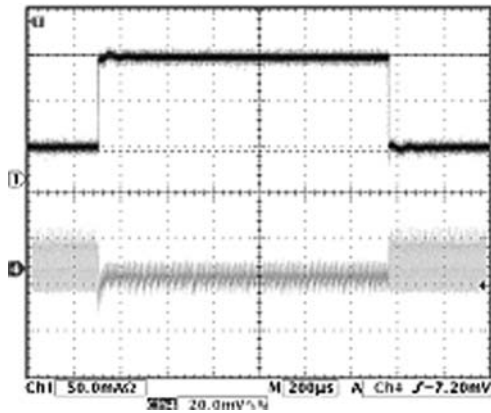
Mode Change by Load Transients V_{OUT} = 1.2V (PWM to PFM)
