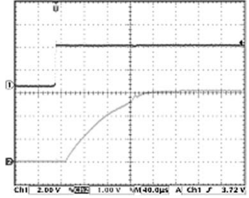
Start up into PFM Mode V_{OUT} = 3.0V, 30\text{ mA load}
