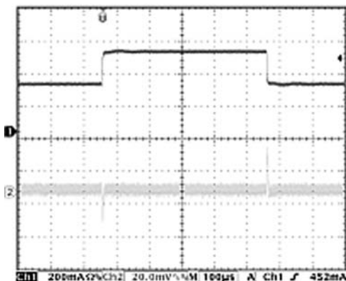
Line Transient Response V_{IN} = 3.6 - 4.2V, V_{OUT} = 1.2V, 250\text{ mA load}
