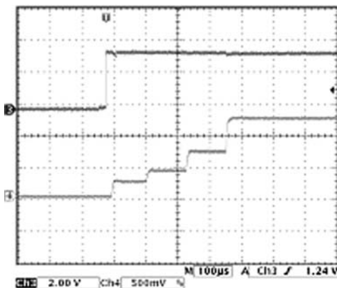
Start up into PWM Mode V_{OUT} = 1.2V, 1.5A\text{ load}
