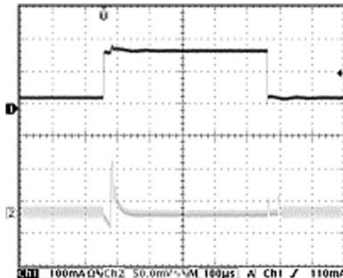
Line Transient Response V_{IN} = 3.0 - 3.6V, V_{OUT} = 3.0V, 250\text{ mA load}
