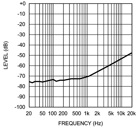
Input Floating
