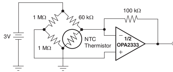
Figure 7. Thermistor Measurement
