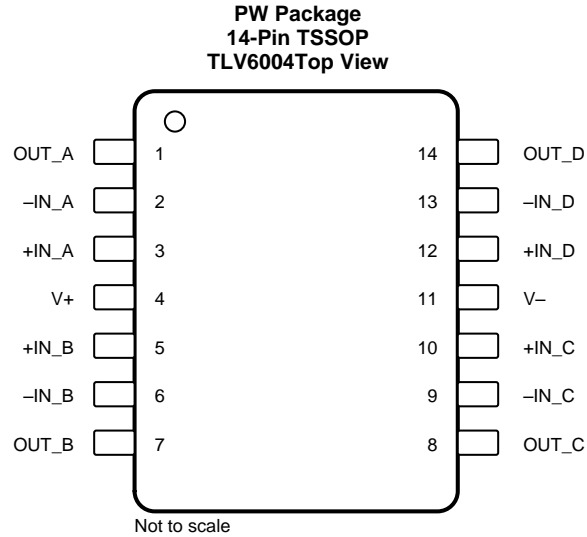
Pin Functions: TLV6004
