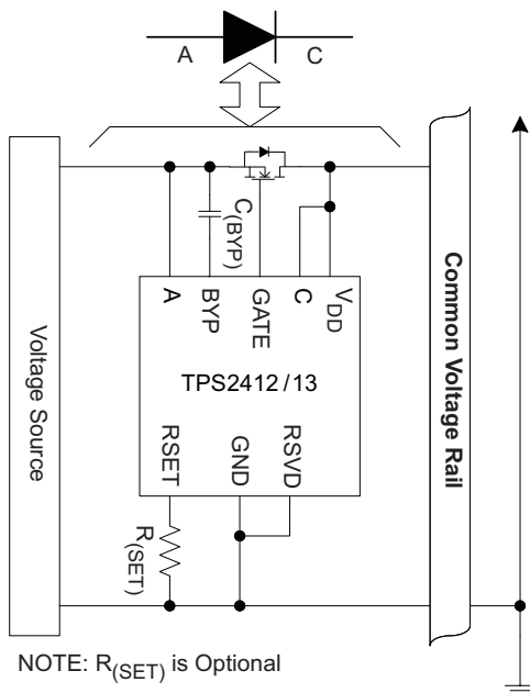
Figure 1. Typical Application
