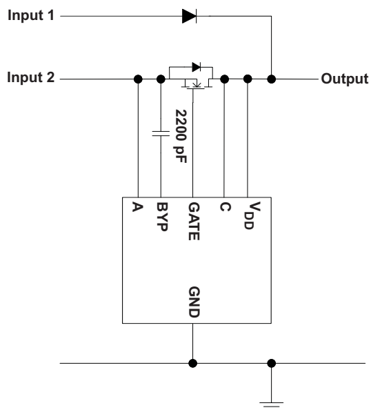
Figure 15. ORing Circuit
