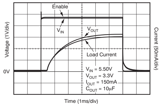
Figure 20. Enable Pin vs Output Voltage Response and Output Current, TPS78233
