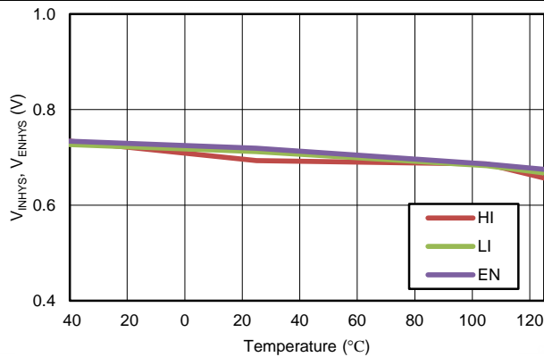
Figure 22. HI/LI/EN Pin Hysteresis vs Temperature
