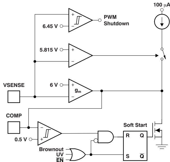
Figure 29. Error Amplifier Block Diagram Showing Speed-Up and Latched Soft-Start
