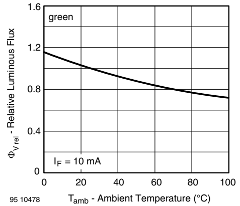
Fig. 17 - Relative Luminous Flux vs. Ambient Temperature
