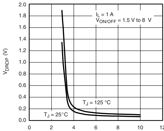
V DR OP vs. V IN at I L = 1 A
