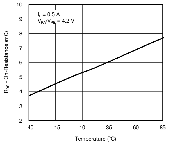
Fig. 8 - On Resistance vs. Temperature
