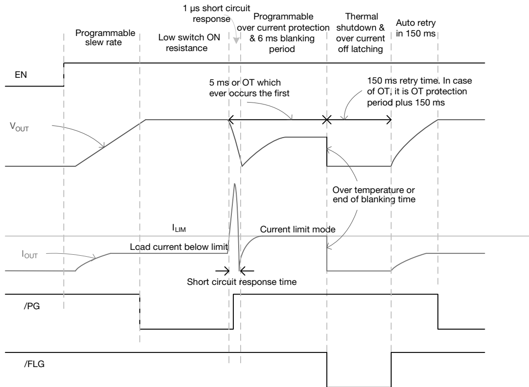
Fig. 2 - Timing Diagram
